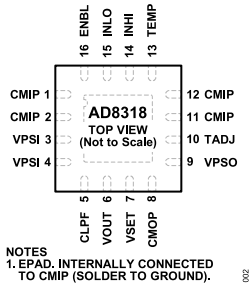
Figure 3. Pin Configuration
