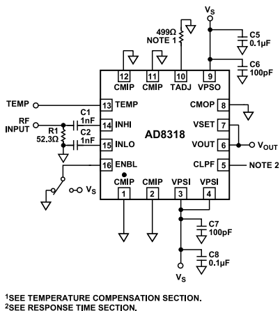
Figure 23. Basic Connections
