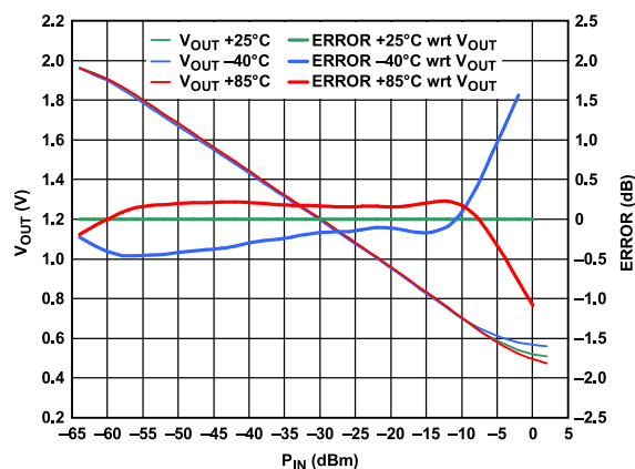
Figure 35. Error vs. Temperature with Respect to Output Voltage at 25^{\circ}\text{C} (Does Not Take Transfer Function Nonlinearities at 25^{\circ}\text{C} into Account)
