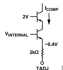
Figure 29. TADJ Interface
