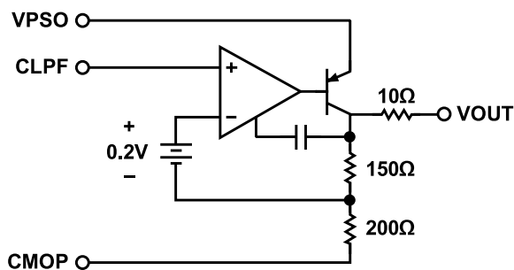
Figure 27. Output Interface
