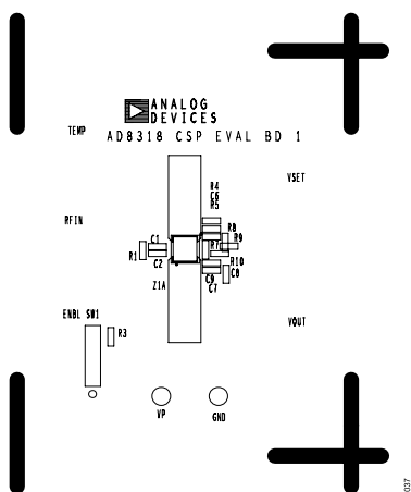
Figure 50. Component Side Silkscreen
