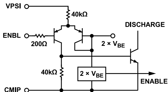
Figure 24. ENBL Interface
