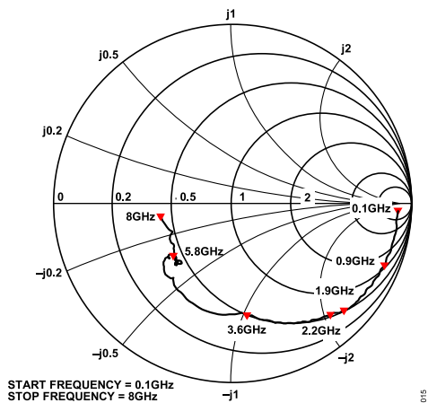
Figure 16. Input Impedance vs. Frequency; No Termination Resistor on INH, Z_0 = 50 \Omega
