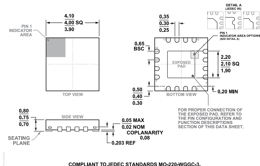
Figure 51. 16-Lead Lead Frame Chip Scale Package [LFCSP] 4 mm × 4 mm Body and 0.75 mm Package Height (CP-16-59) Dimensions shown in millimeters
