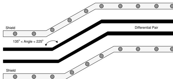
Figure 10-13. FPD-Link Routing Example
