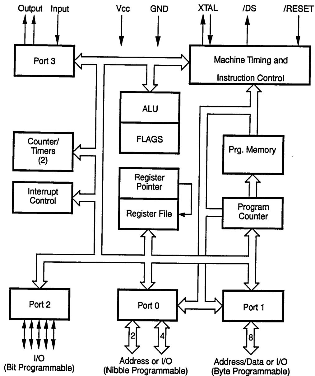
Figure 1. Z86C60/65 Functional Block Diagram
