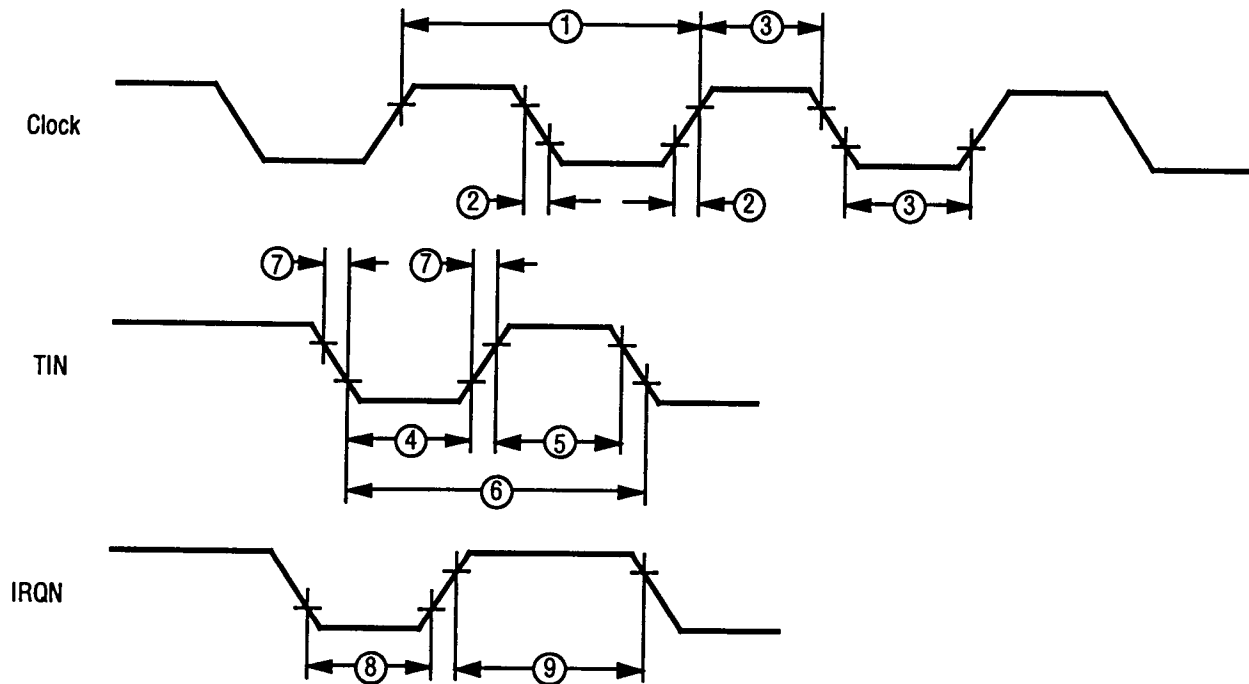
Figure 4. Additional Timing
