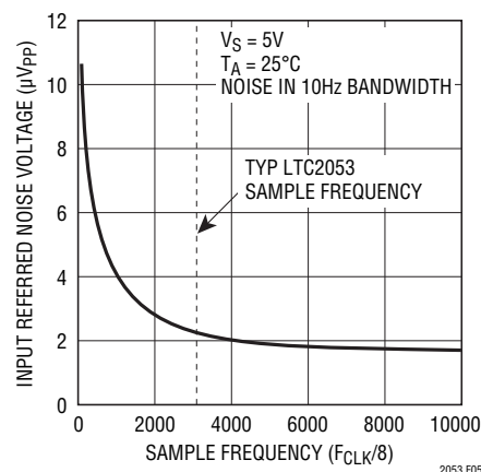
Figure 5. LTC2053-SYNC Input Referred Noise vs Sample Frequency
