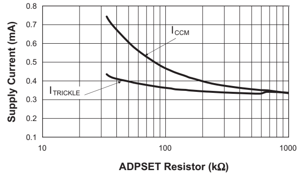
Adapter Mode Supply Current vs. ADPSET Resistor
