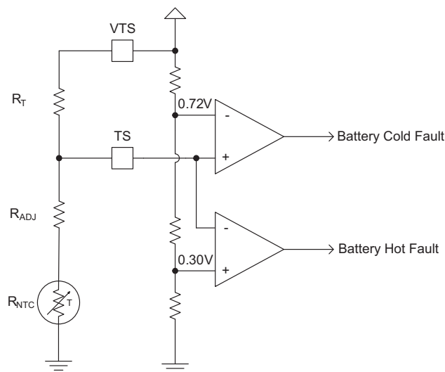
Figure 7: Battery Temperature Sense Circuit with Externally Adjusted Window Threshold.
