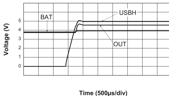
Transient Response of OUT When Switching From BAT to USBH ( V_{USBH} = 0V \rightarrow 5V ; R_{LOAD} = 7.8\Omega )
