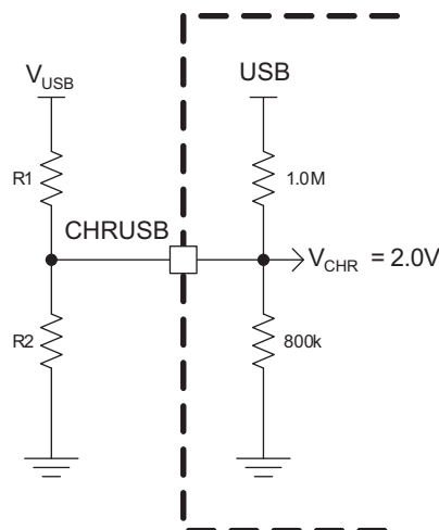
Figure 4: Internal Equivalent Circuit for the CHRUSB Pin.
