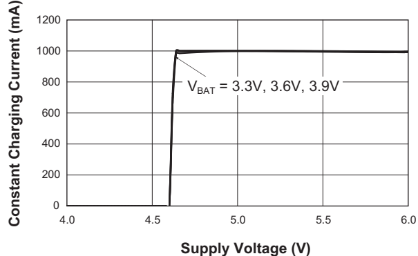
Constant Charging Current vs. Supply Voltage (ADP; CHRADP = Open; ADPSET = 57.6k \Omega )
