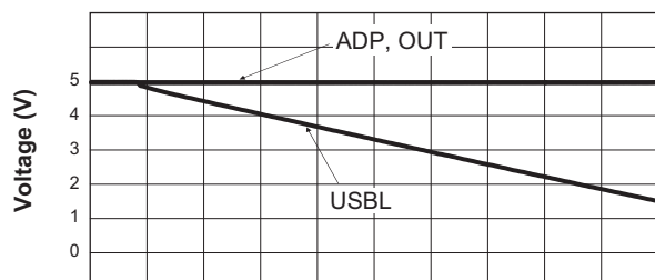
Transient Response of OUT When Switching From ADP to USBL ( V_{\text{USBL}} = 5\text{V} \rightarrow 0\text{V} ; R_{\text{LOAD}} = 50\Omega )
