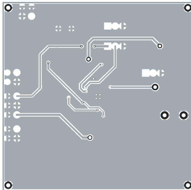
Figure 10: AAT3670 Evaluation Board Bottom Side Layout.
