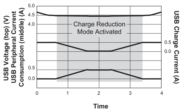
USB Charge Current vs. Time (USBH)
