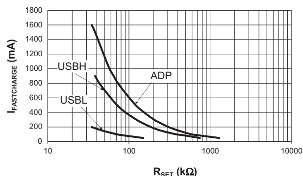
Figure 5: Fast Charge Current vs. Set Resistor ( V_{IN} = 5V ; V_{BAT} = 3.5V ).
