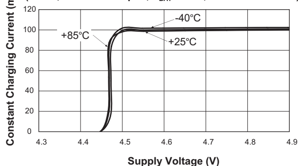
Constant Charging Current vs. Supply Voltage (USBL; CHRUSB = Open; V BAT = 3.6V; USBSET = 71.5k \Omega )
