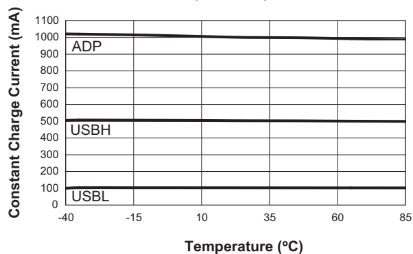
Constant Charge Current vs. Temperature (V IN = 5.0V)
