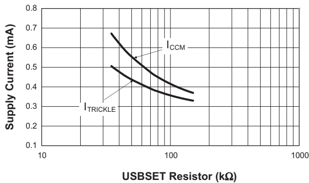
USB Mode Supply Current vs. USBSET Resistor
