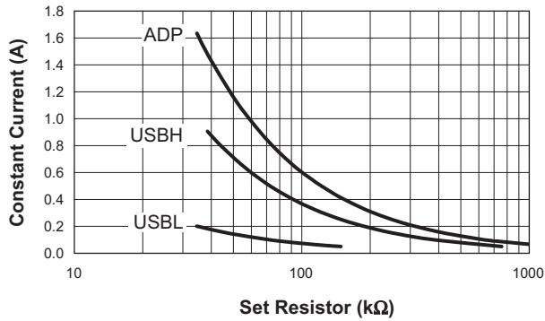
Constant Current vs. Set Resistor
