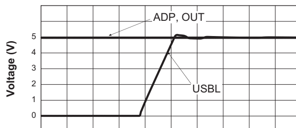
Transient Response of OUT When Switching From USBL to ADP ( V_{\text{USBL}} = 0\text{V} \rightarrow 5\text{V} ; R_{\text{LOAD}} = 50\Omega )
