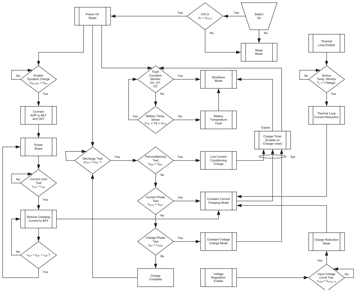
Figure 2: AAT3670 Operational Flow Chart.
