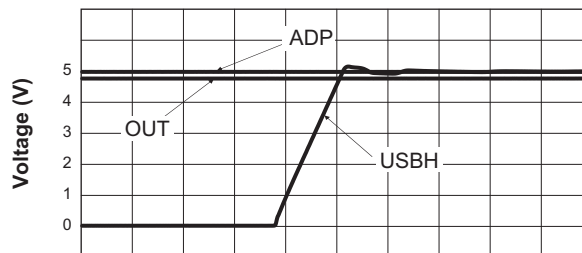
Transient Response of OUT When ADP is On When USBH Switching from Off to On ( V_{\text{USBH}} = 0\text{V} \rightarrow 5\text{V} ; R_{\text{LOAD}} = 7.8\Omega )
