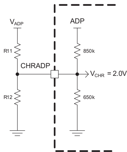
Figure 3: Internal Equivalent Circuit for the CHRADP Pin.
