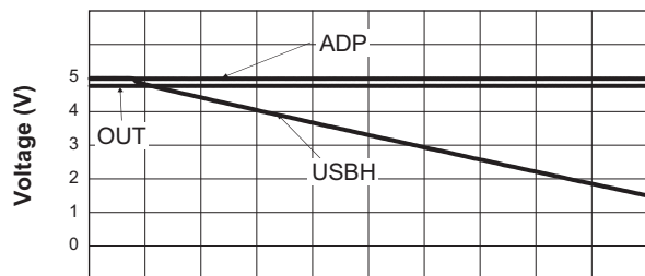
Transient Response of OUT When ADP is On When USBH Switching from On to Off ( V_{\text{USBH}} = 5\text{V} \rightarrow 0\text{V} ; R_{\text{LOAD}} = 7.8\Omega )
