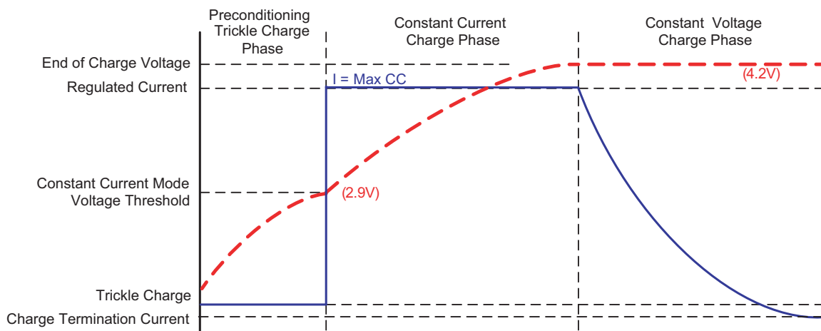
Figure 1: Current vs. Voltage Profile During Charging Phases.
