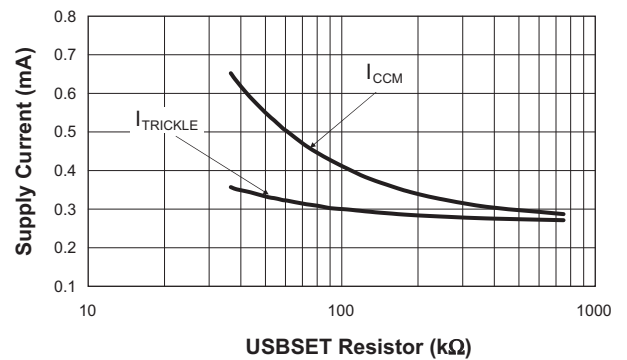
USB Mode Supply Current vs. USBSET Resistor
