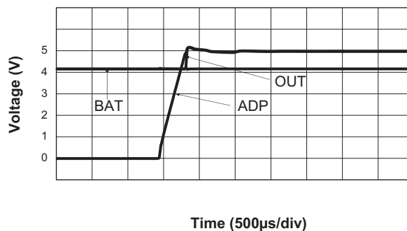
Transient Response of OUT When Switching from BAT to ADP ( V_{ADP} = 0V \rightarrow 5V )
