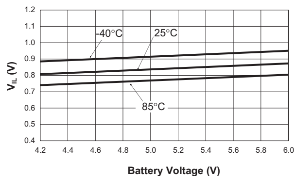
V_{IL} vs. Supply Voltage (ENBAT = Falling)
