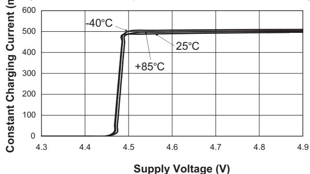
Constant Charging Current vs. Supply Voltage (USBH; CHRUSB = Open; V BAT = 3.6V; USBSET = 71.5k \Omega )
