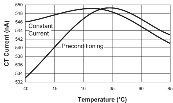
CT Current vs. Temperature ( C_T = 0.1\mu F )
