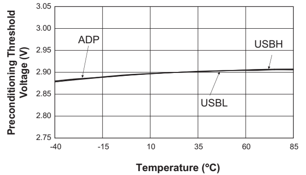
Preconditioning Threshold Voltage vs. Temperature ( V_{IN} = 5.0V )
