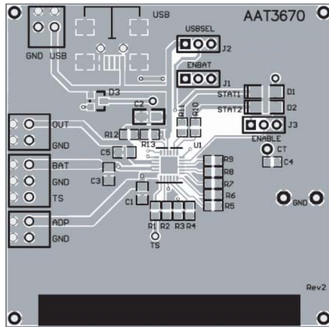
Figure 9: AAT3670 Evaluation Board Top Side Layout.
