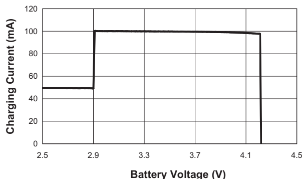
Charging Current vs. Battery Voltage (USBL; USBSET = 71.5k \Omega )
