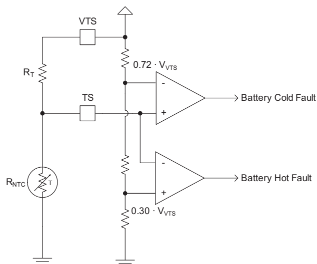
Figure 6: Battery Temperature Sense Circuit.
