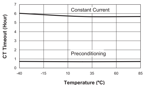
CT Timeout vs. Temperature ( C_T = 0.1\mu F )
