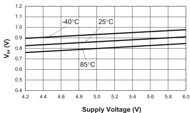
V_{IH} vs. Supply Voltage (ADP or USBL or USBH; EN = Rising)
