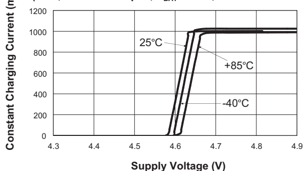
Constant Charging Current vs. Supply Voltage (ADP; CHRADP = Open; V BAT = 3.6V; ADPSET = 57.6k \Omega )
