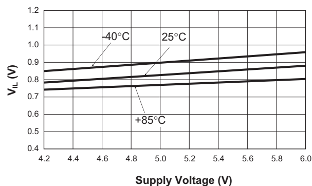
V_{IL} vs. Supply Voltage (ADP or USBL or USBH; EN = Falling)
