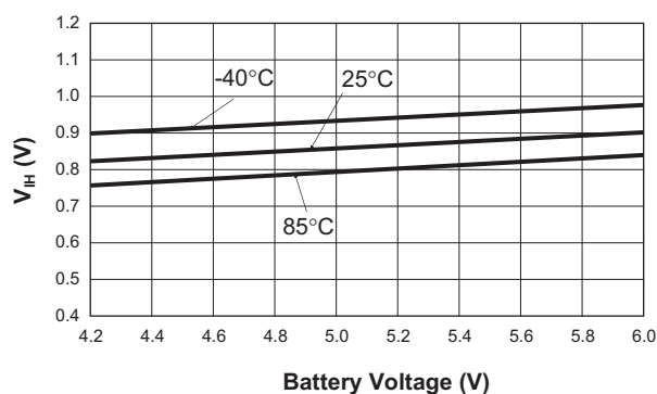
V_{IH} vs. Supply Voltage (ENBAT = Rising)
