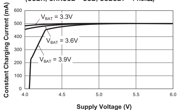
Constant Charging Current vs. Supply Voltage (USBH; CHRUSB = USB; USBSET = 71.5k \Omega )
