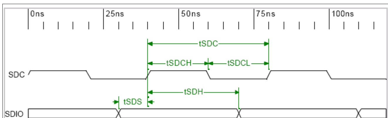
Figure 7 SMI Timing
