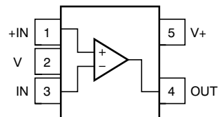
OPA333 DCK Package 5-Pin SC70 Top View
