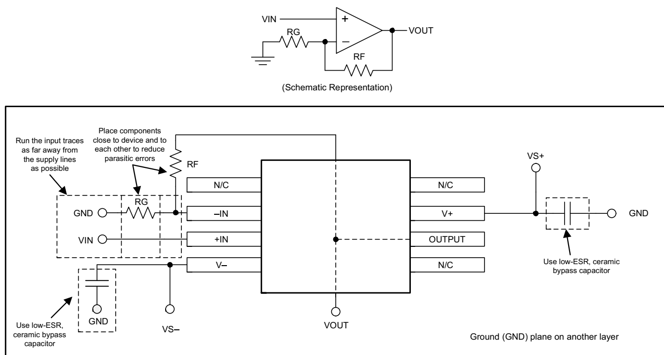
Figure 34. Layout Example
