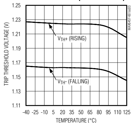
TRIP THRESHOLD VOLTAGE vs. TEMPERATURE (5% HYSTERESIS)
