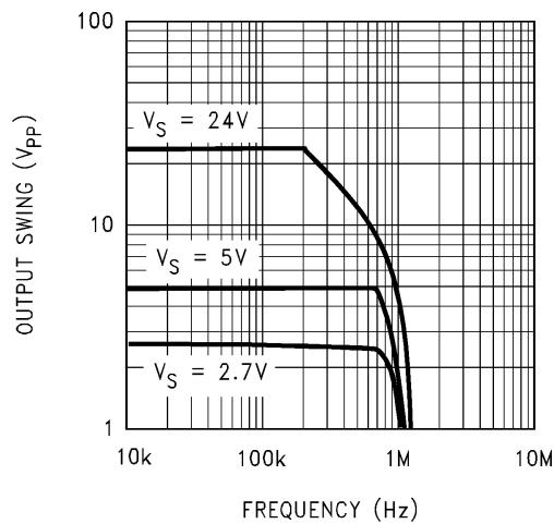
Voltage Swing vs. Frequency ( C_L = 100\text{ pF} )
