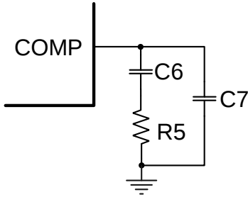
Figure 9: Compensation Network
