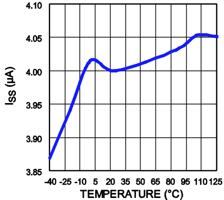
Soft-Start Source Current vs. Temperature
