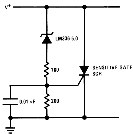
Figure 15. 5V Crowbar
