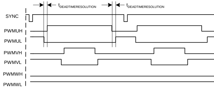
Figure 12: PWM Timing
