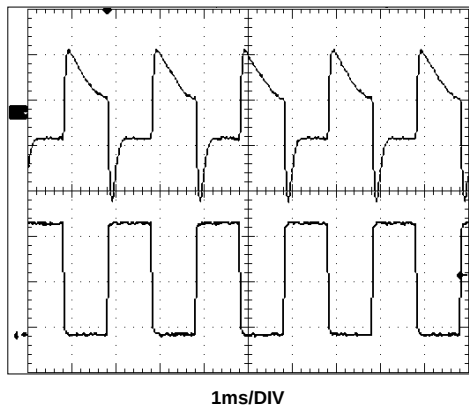
FIGURE 3. A_{VDD} TRANSIENT RESPONSE
