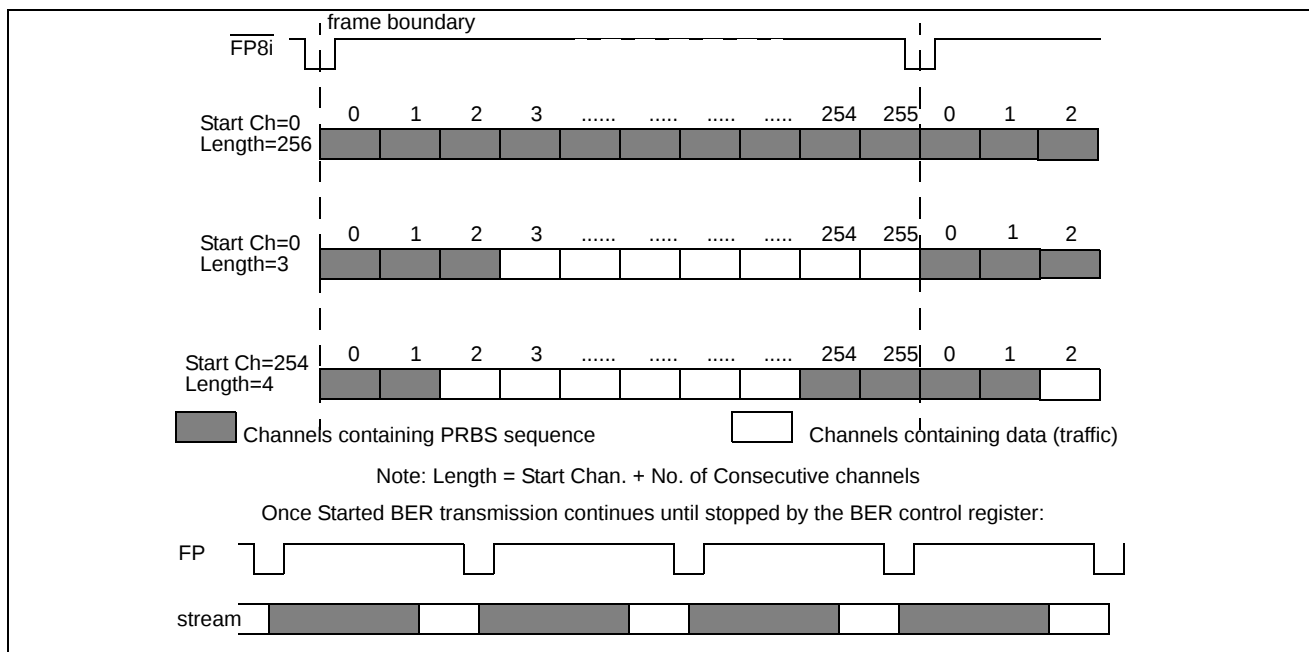
Figure 17 - Examples of BER transmission channels
