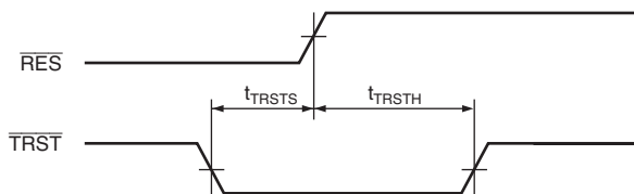
Figure 21.52 TCK Input Timing in Reset Hold State
