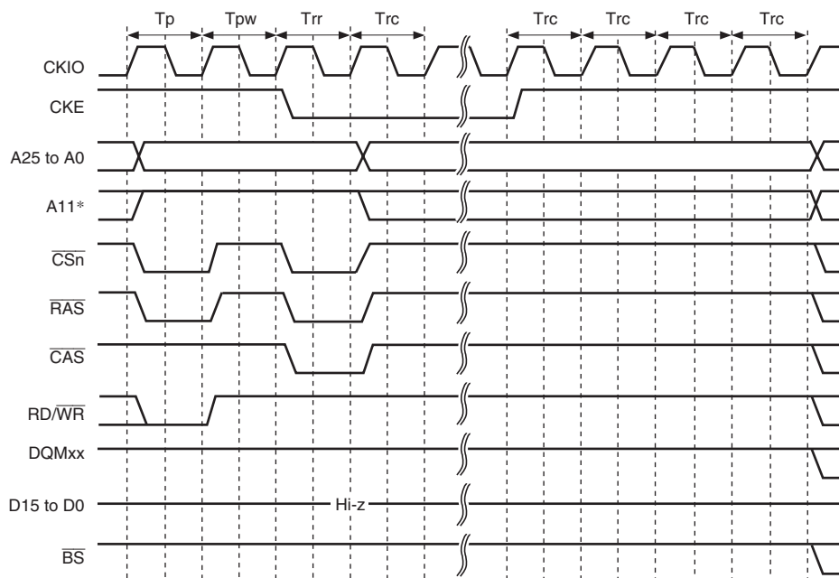
Figure 7.24 Self-Refreshing Timing
