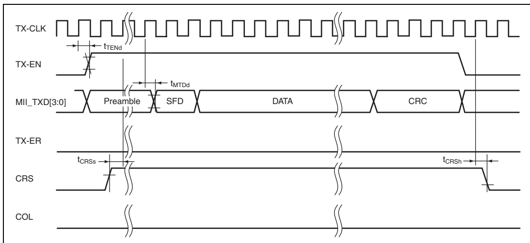
Figure 21.43 MII Transmission Timing (Normal Operation)
