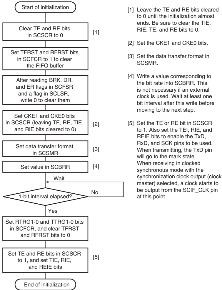
Figure 14.12 Sample Flowchart for SCIF Initialization
