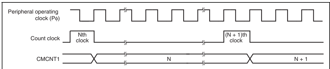
Figure 13.3 Count Timing
