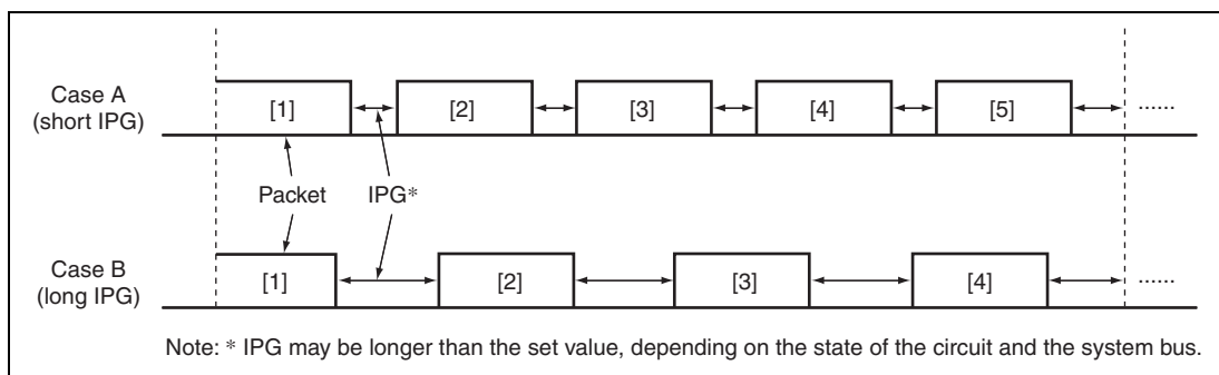
Figure 11.7 Changing IPG and Transmission Efficiency
