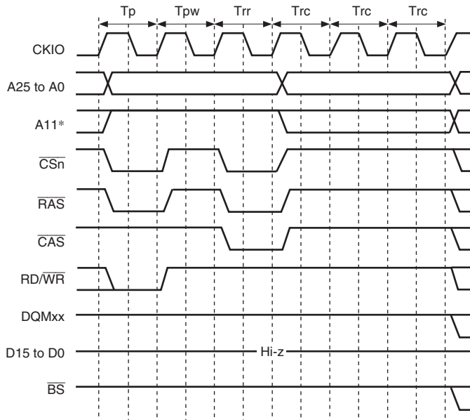
Figure 7.23 Auto-Refreshing Timing
