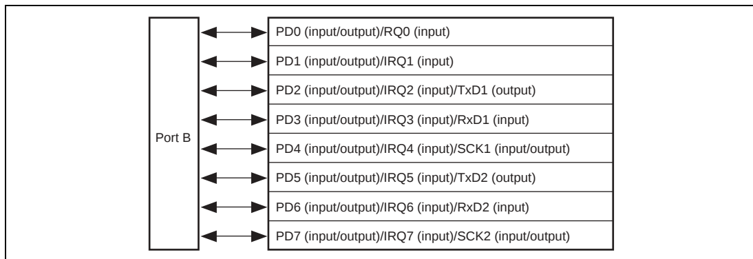
Figure 17.4 Port D
