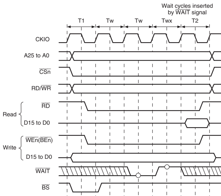
Figure 7.9 Wait Cycle Timing for Normal Space Access (Wait cycle Insertion using \overline{WAIT} )
