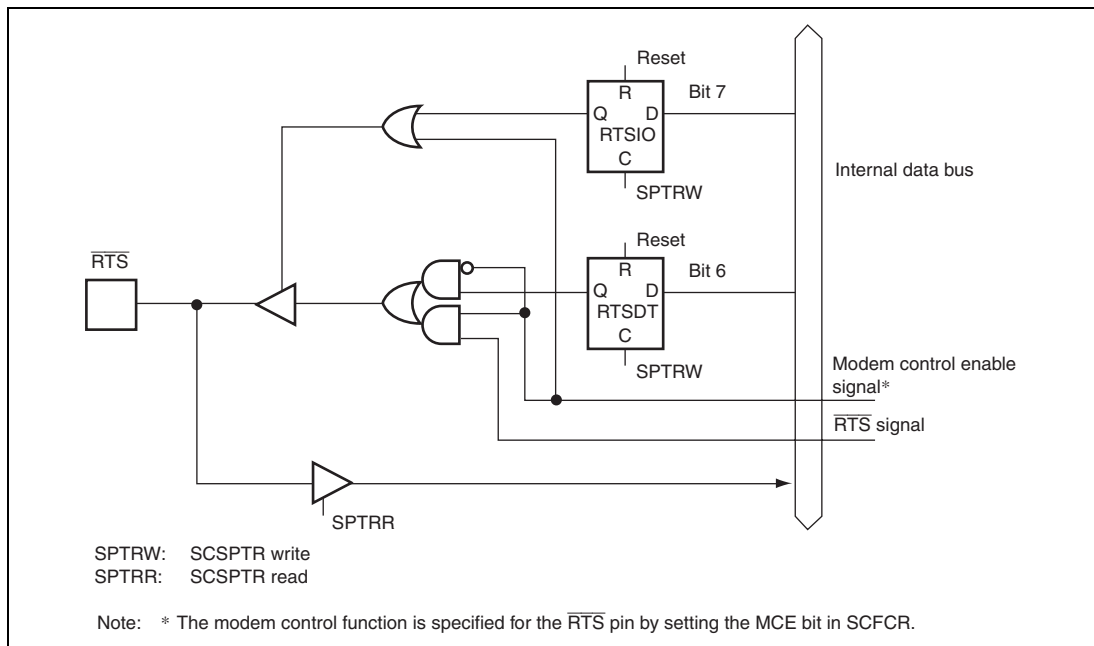
Figure 14.19 RTSIO Bit, RTSDT bit, and \overline{\text{RTS}} Pin
