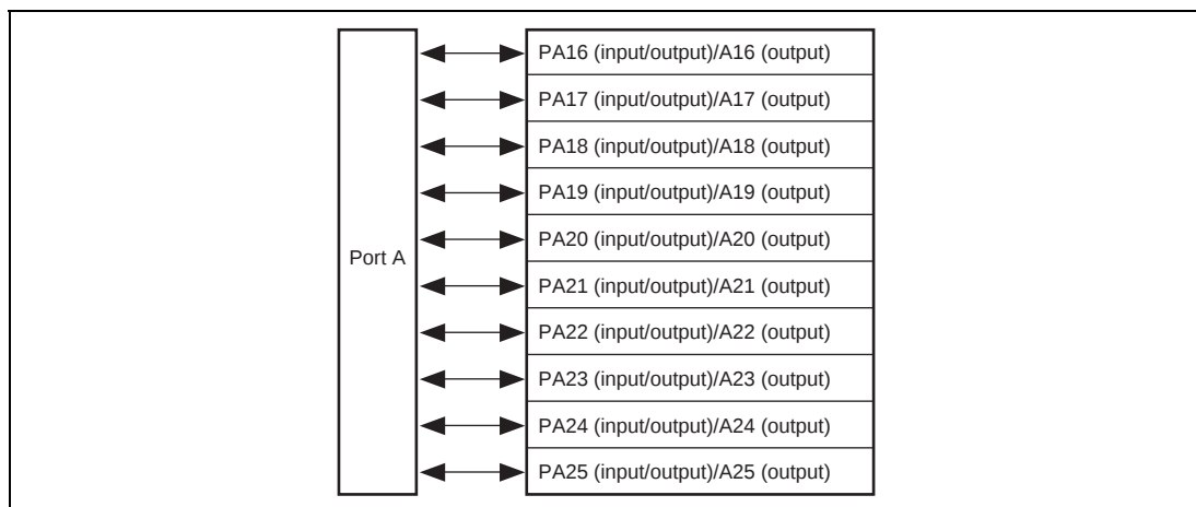
Figure 17.1 Port A
