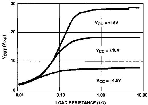
FIGURE 34. OUTPUT SWING vs LOAD RESISTANCE
