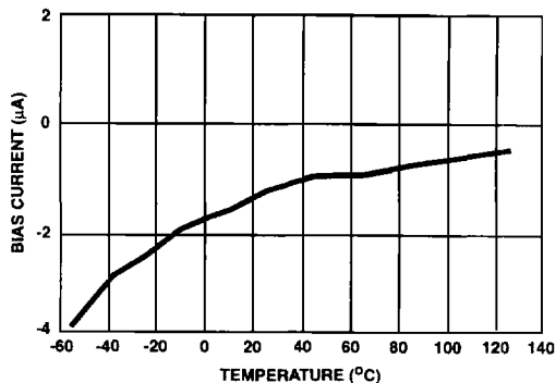
FIGURE 27. +INPUT BIAS CURRENT vs TEMPERATURE
