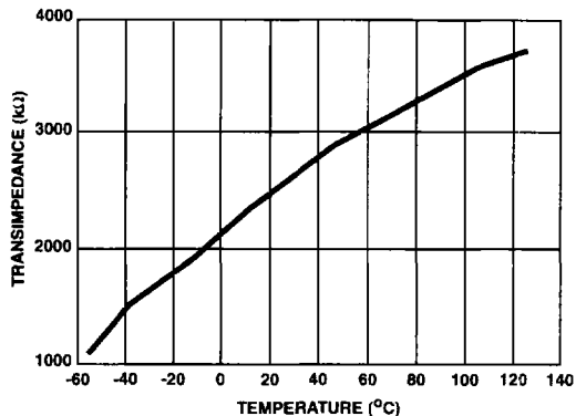
FIGURE 29. TRANSIMPEDANCE vs TEMPERATURE
