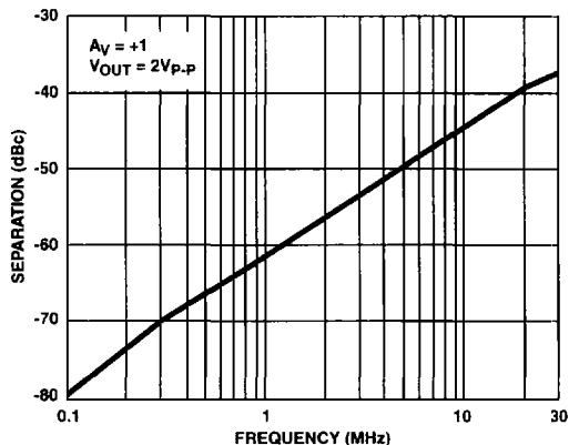
FIGURE 37. CHANNEL SEPARATION vs FREQUENCY
