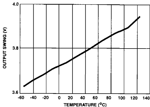
FIGURE 33. OUTPUT SWING vs TEMPERATURE
