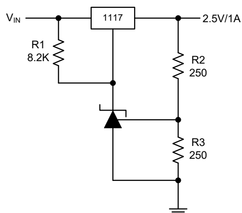
Figure 7. Precision 2.5V/1A Regulator
