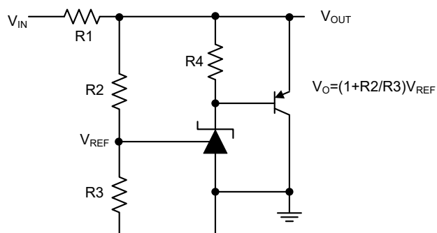
Figure 5. High Current Shunt Regulator
