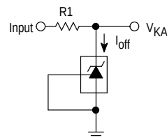
Figure 3. Test Circuit for I_{off}
