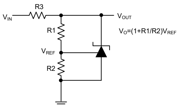
Figure 4. Shunt Regulator
