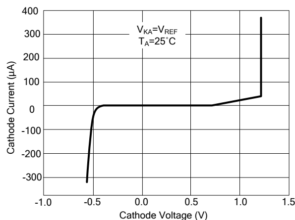
Figure 12. Current VS. cathode Voltage
