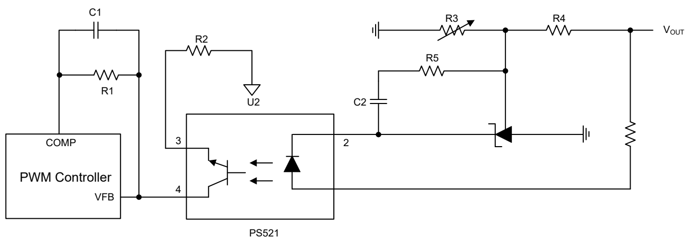
Figure 8. PWM Converter with Reference
