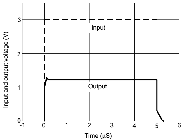
Figure 15. Pulse Response of Input and Output Voltage
