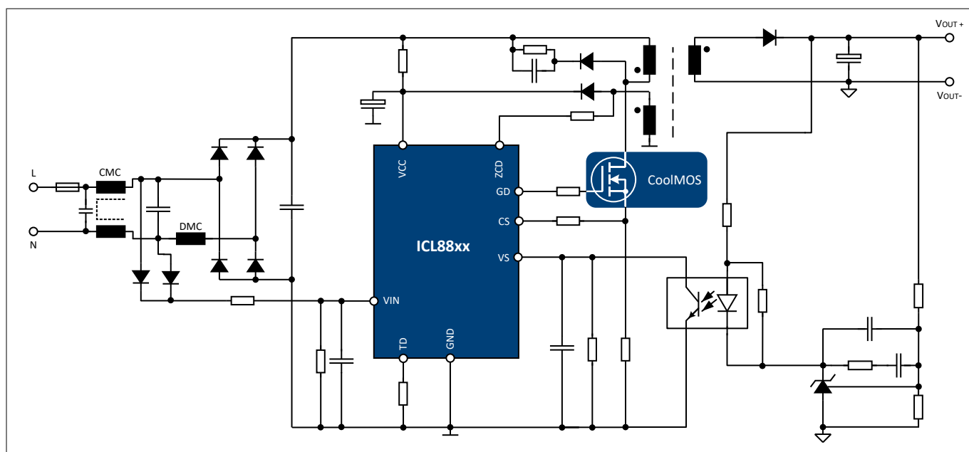
Figure 1 Flyback-SSR-CV
