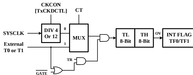
Figure 6 Timer 0 and 1 Mode 1 Block Diagram
