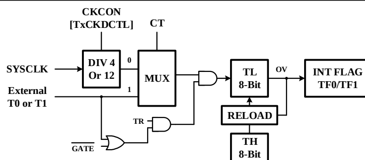
Figure 7 Timer 0 and 1 Mode 2 Block Diagram
