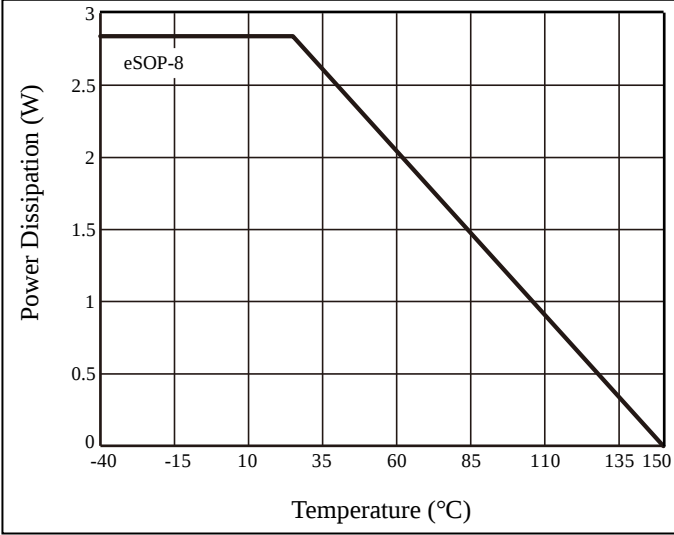
Figure 27 Dissipation Curve
