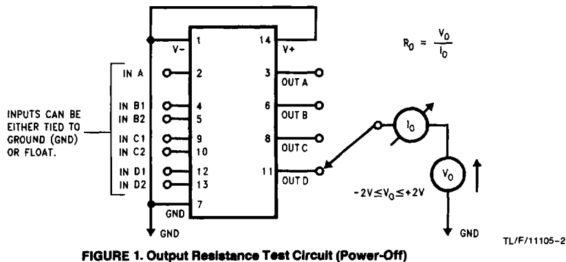
FIGURE 1. Output Resistance Test Circuit (Power-Off)
