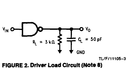
FIGURE 2. Driver Load Circuit (Note 8)
