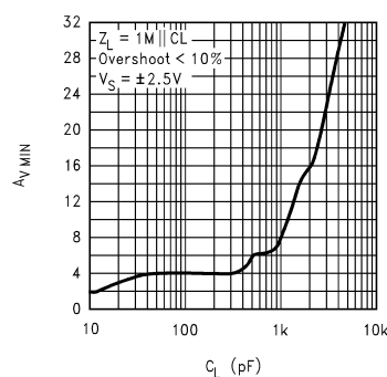
FIGURE 4. Minimum Operating Gain vs Capacitive Load
