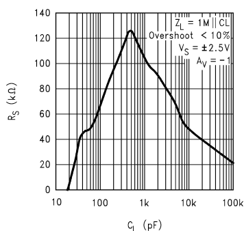
FIGURE 5. Isolating Resistor Value vs Capacitive Load
