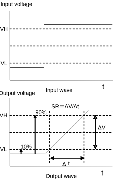
Figure 53. Slew Rate Input Waveform
