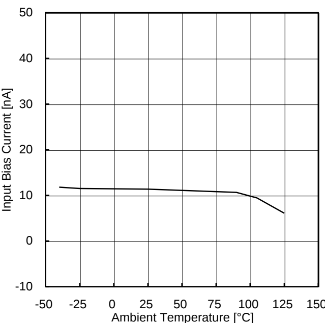
Figure 41. Input Bias Current vs Ambient Temperature ( V_{CC}=30V , V_{ICM}=28V , E_K=-1.4V )
