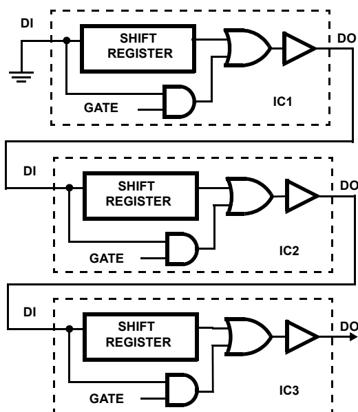
FIGURE 3. CASCADED CHIP OPERATION TO READ DIAGNOSTIC DATA
