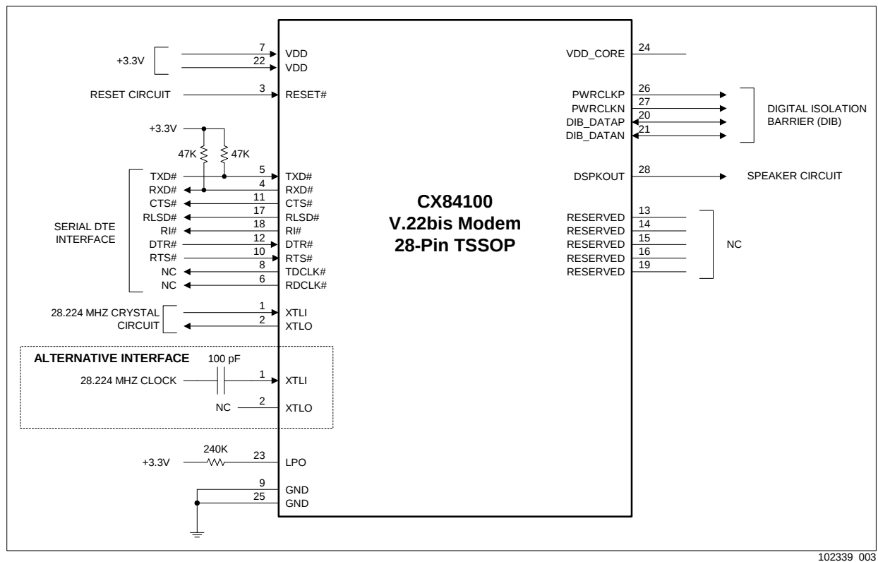
Figure 3-1. CX84100 V.22bis Modem Hardware Interface Signals
