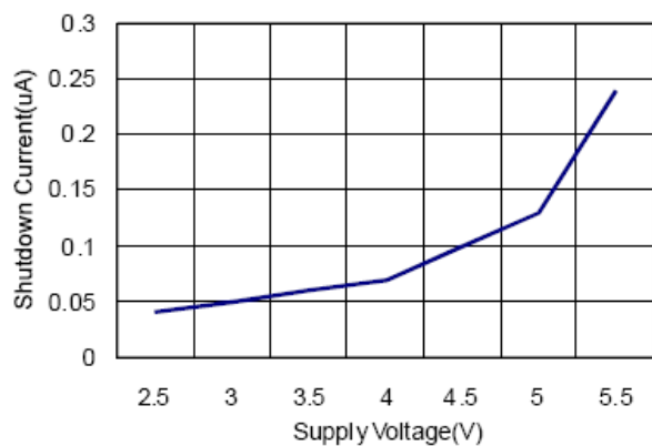
27. Shutdown Current
