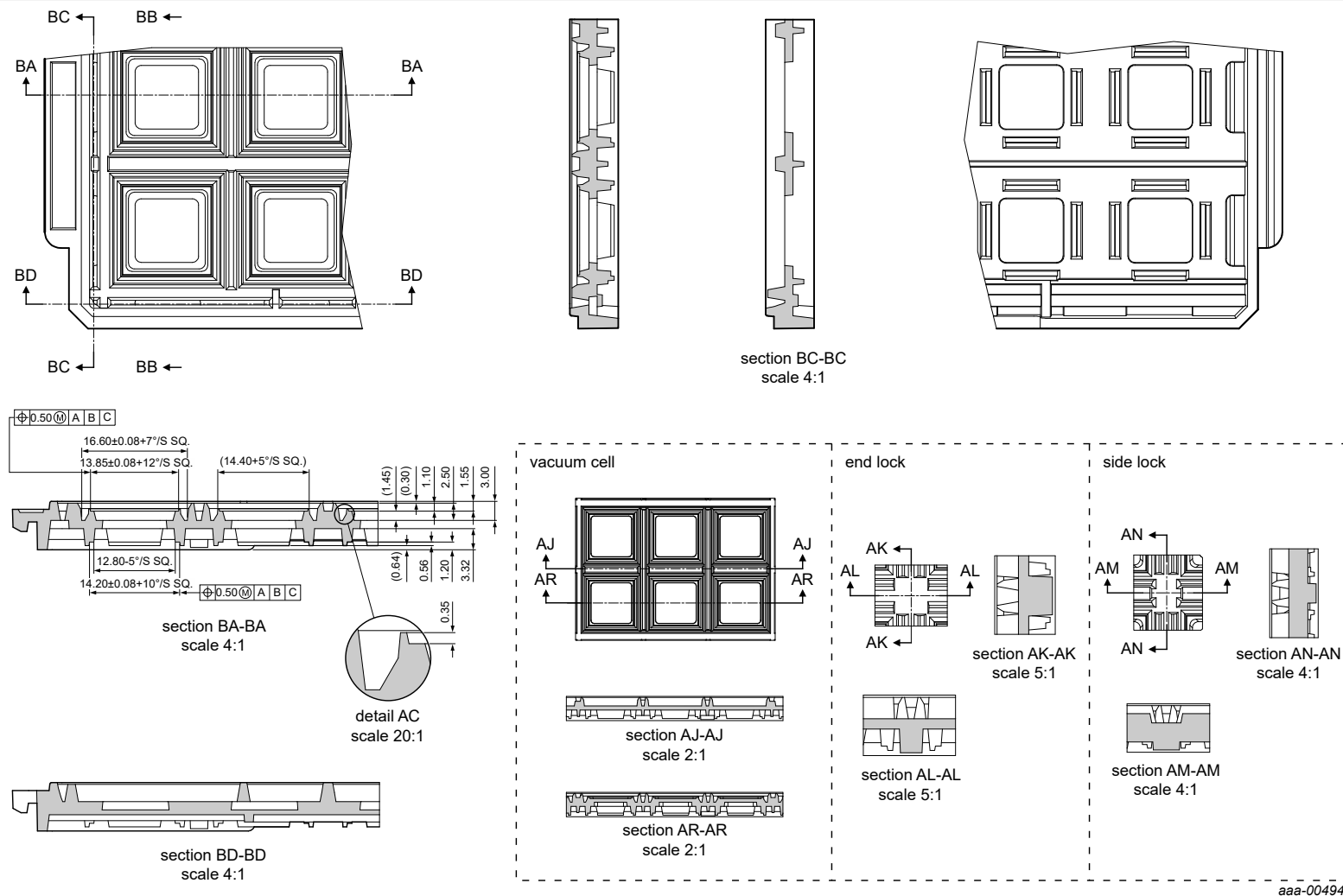
Figure 35. Tray details
