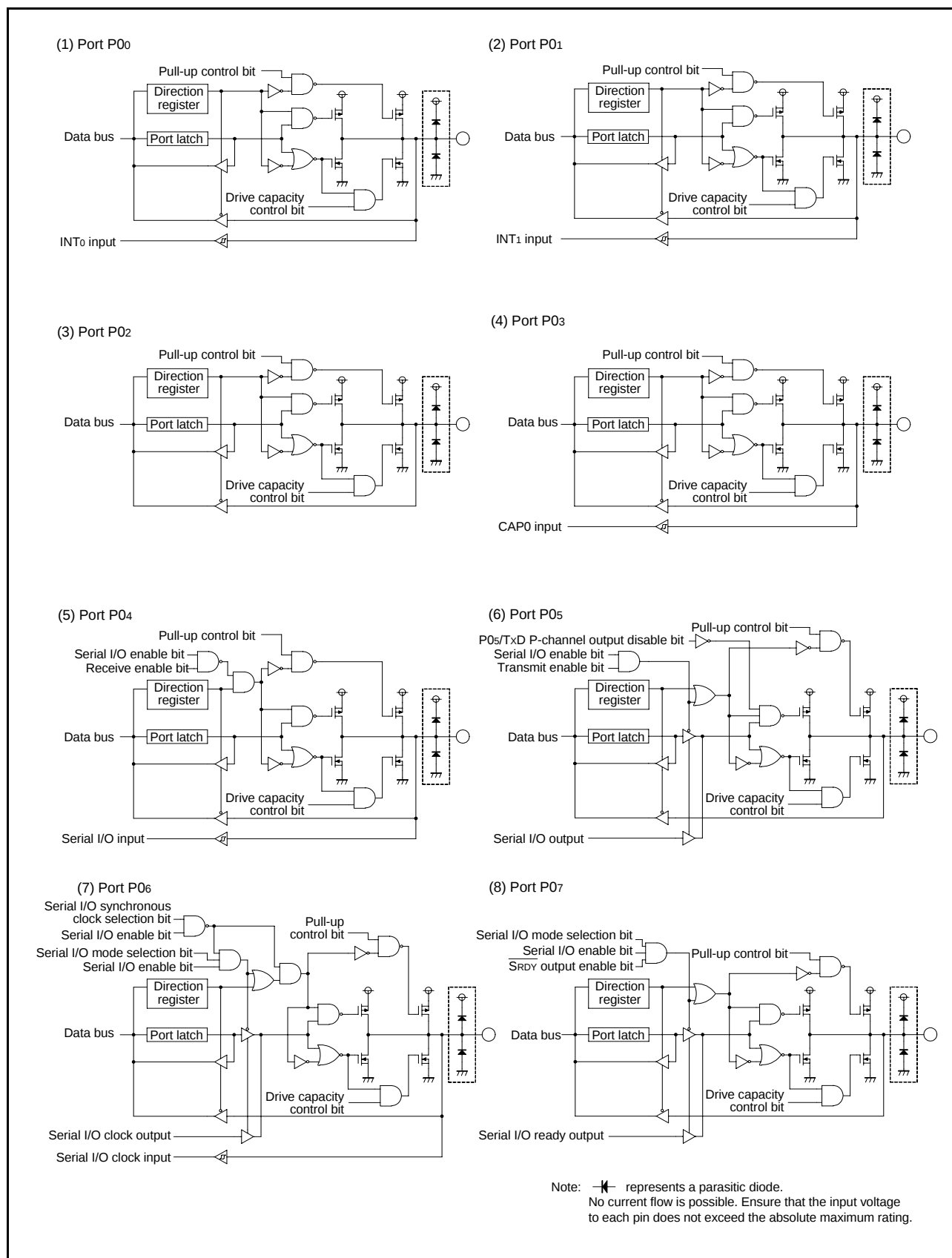
Fig 17. Block diagram of pins (1)
