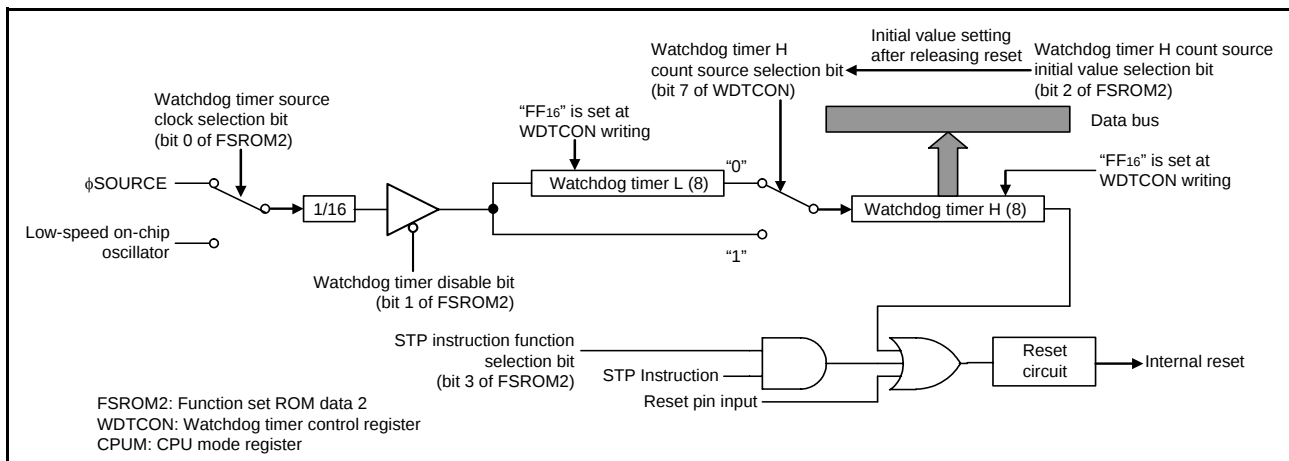
Fig 56. Block diagram of watchdog timer
