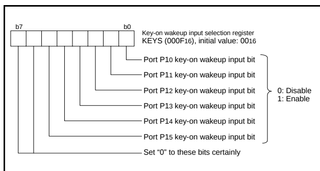
Fig 25. Structure of key input control register
