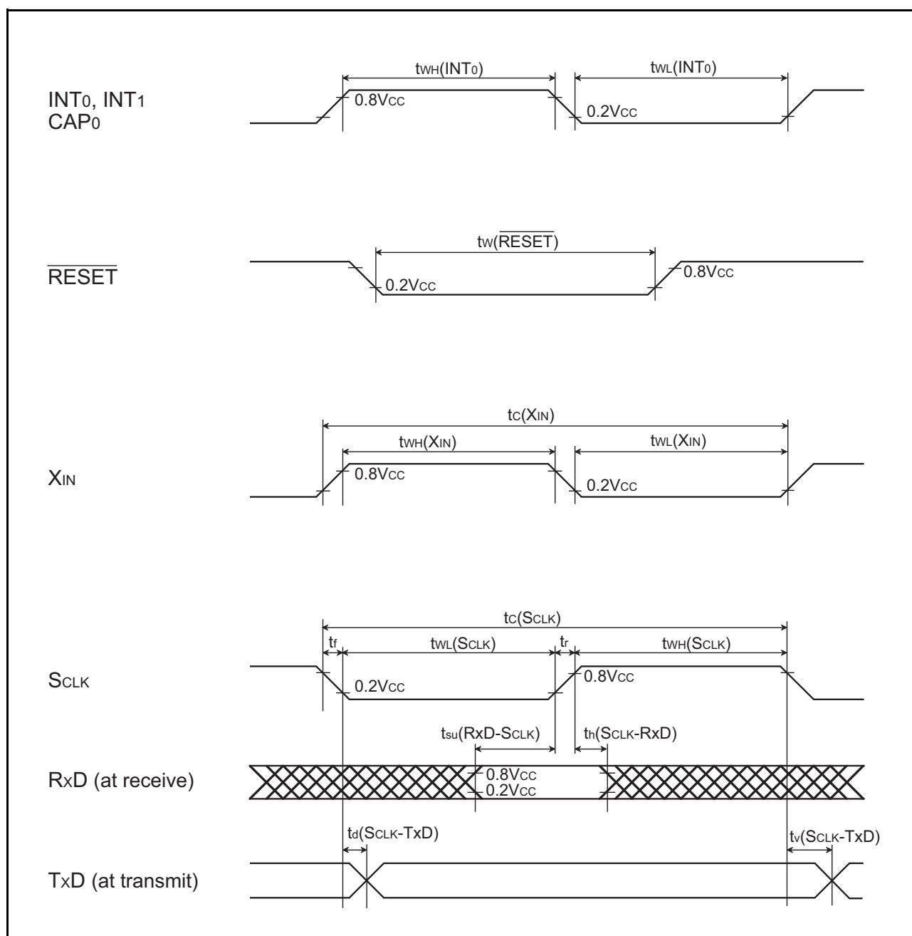
Fig 86. Timing chart
