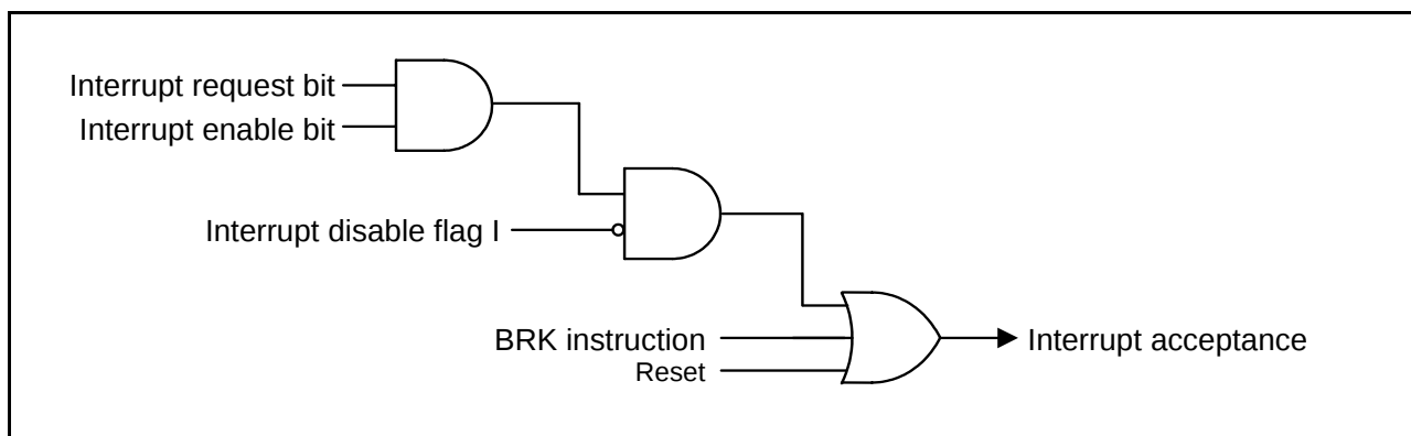
Fig 19. Interrupt control
