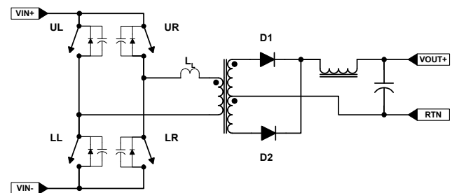
FIGURE 10. IDEALIZED FULL-BRIDGE
