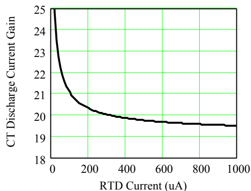
FIGURE 2. CT DISCHARGE CURRENT GAIN vs RTD CURRENT
