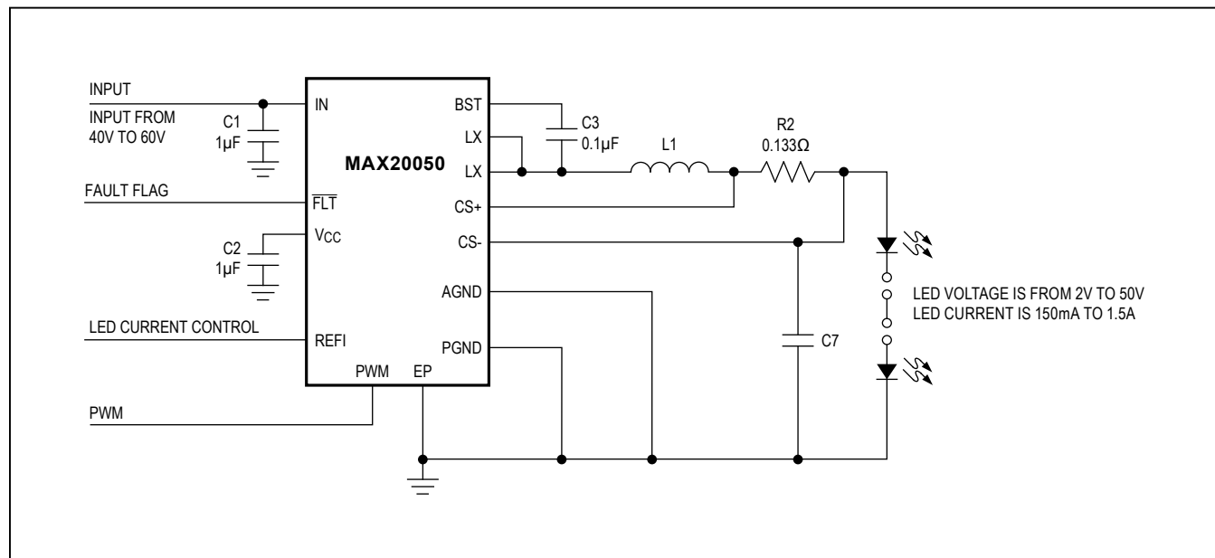
Figure 7. Typical Input Voltage (50V)
