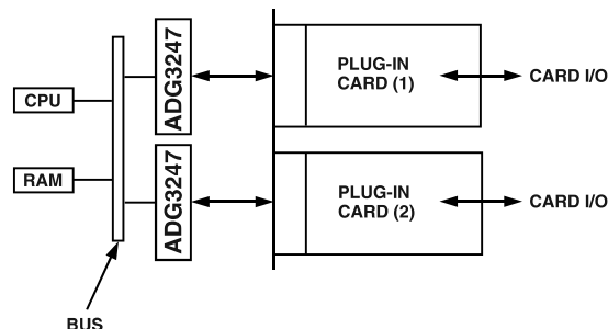
Figure 12. ADG3247 in a Hot Plug Application
