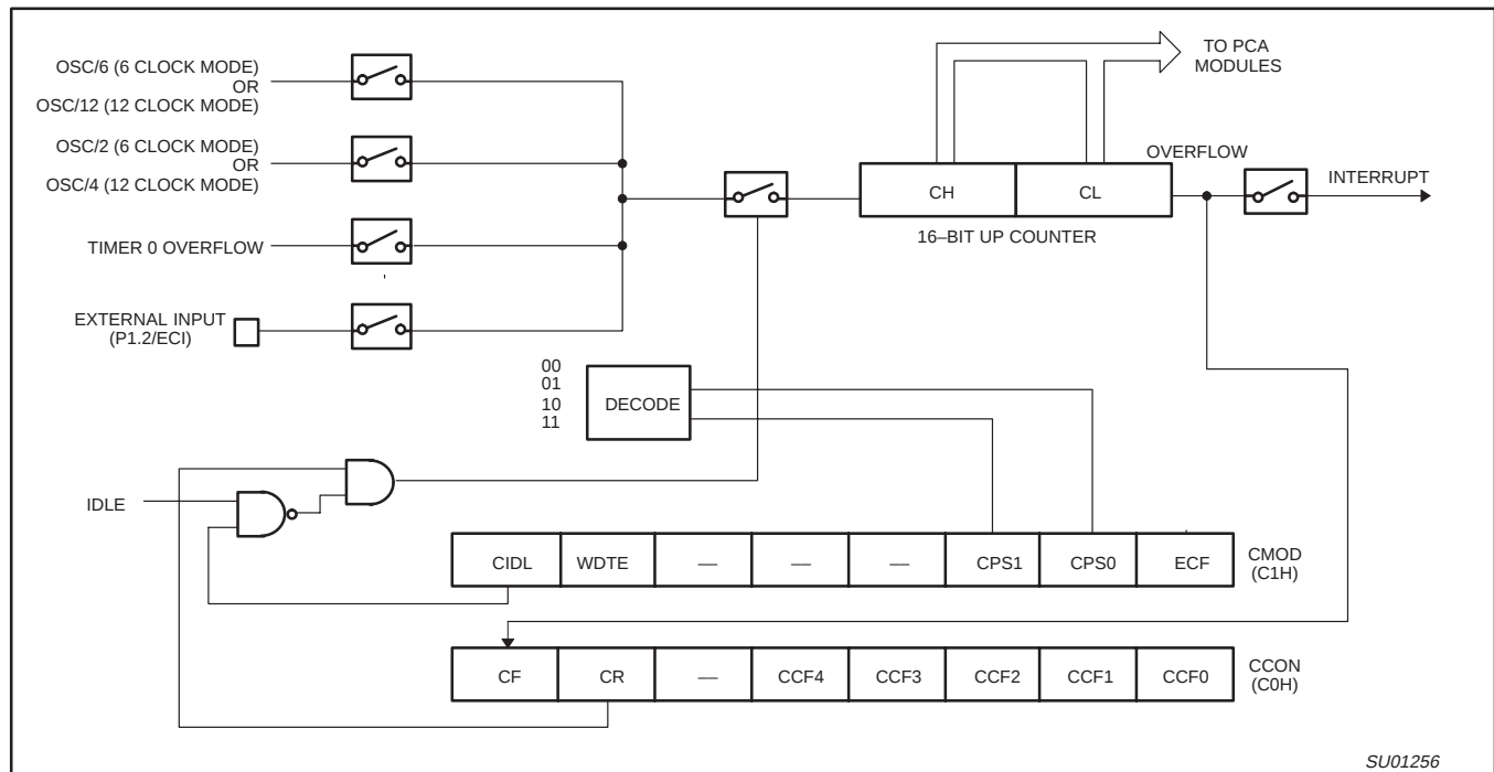
Figure 36. PCA Timer/Counter
