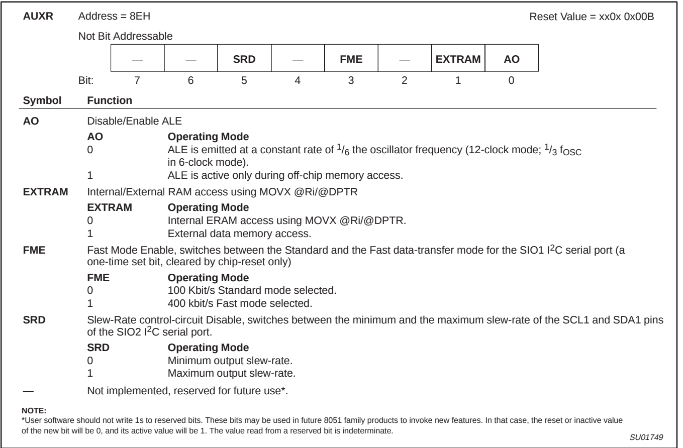
Figure 48. AUXR: Auxiliary Register
