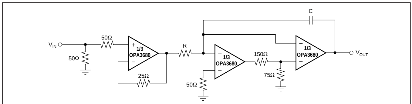
FIGURE 7. Wideband Integrator.
