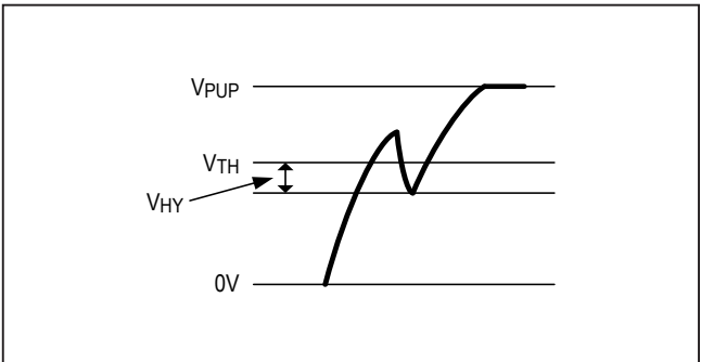
Figure 6. Noise Suppression Scheme
