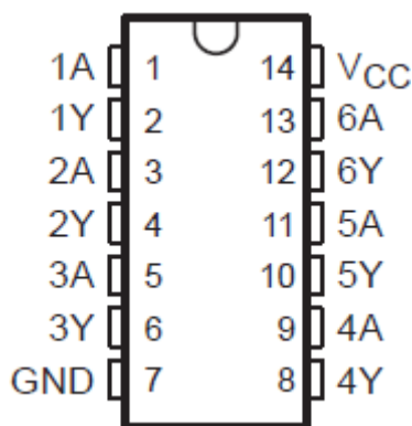
Figure 4-1. CD54AC04 F Package, CD74AC04 E or M Package, Top View
