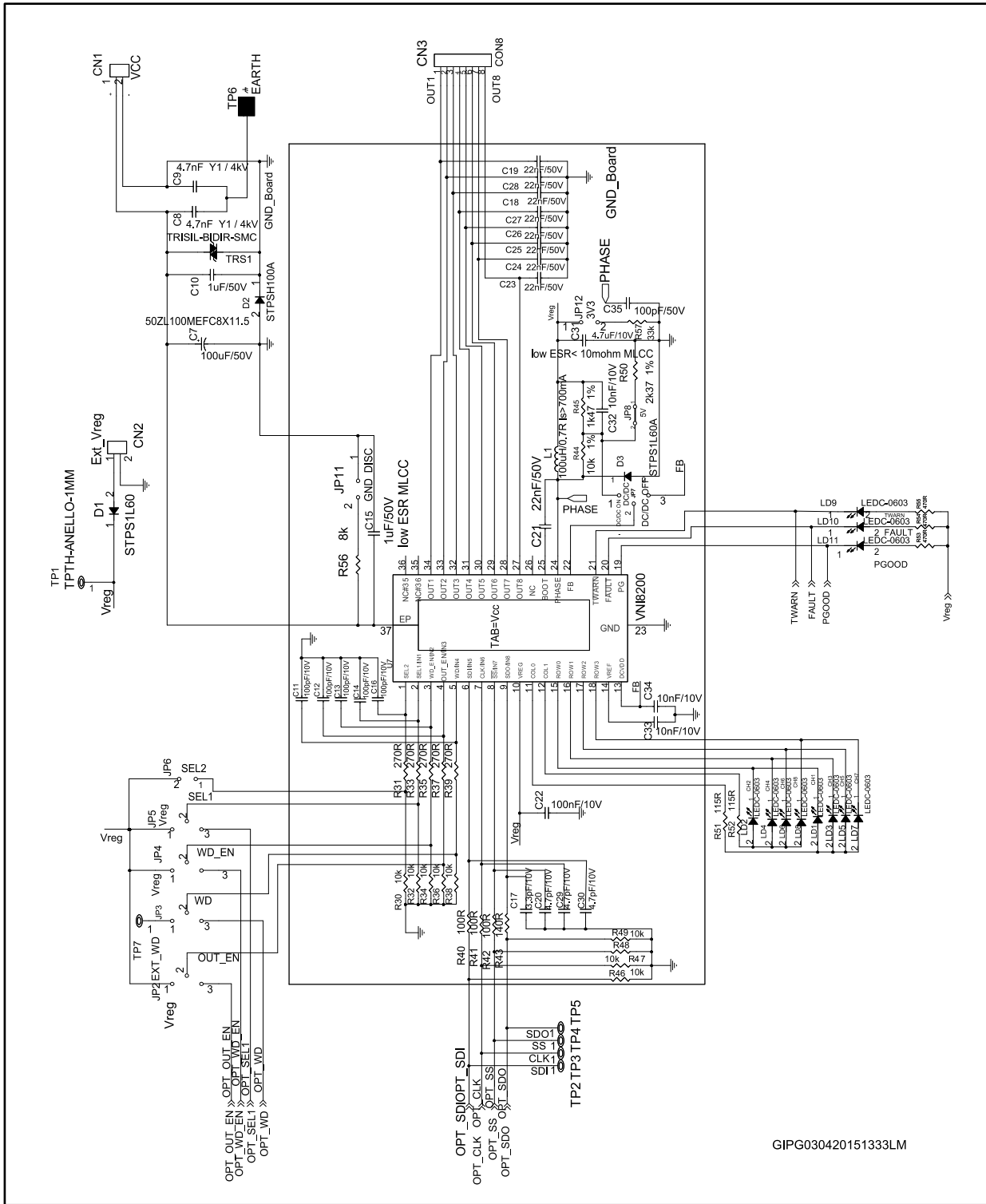
Figure 11: Typical circuit for switching regulation V_{DC-out} = 5\text{ V}
