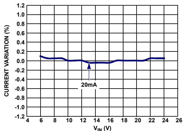
FIGURE 5. CURRENT REGULATION
