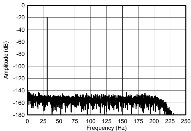
Figure 6-24. Mid-Power Mode FFT Spectrum
