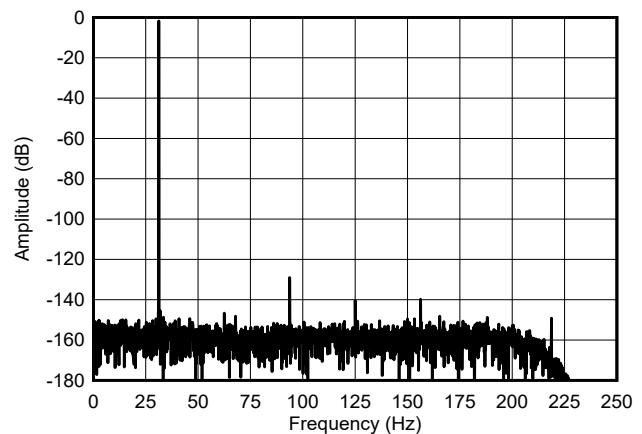
Figure 6-28. Low-Power Mode FFT Spectrum
