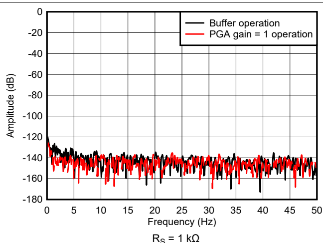
Figure 6-12. High-Power Mode FFT Spectrum
