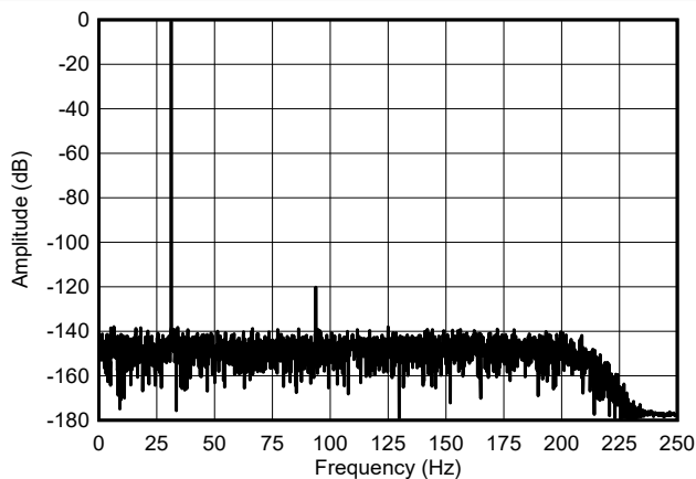
Figure 6-23. Mid-Power Mode FFT Spectrum
