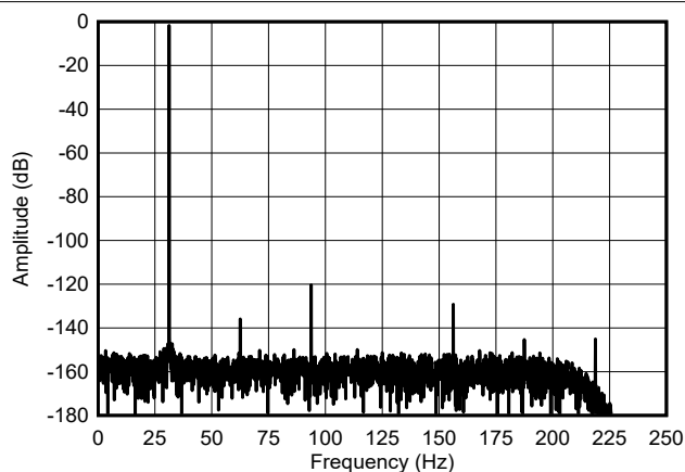
Figure 6-22. Mid-Power Mode FFT Spectrum
