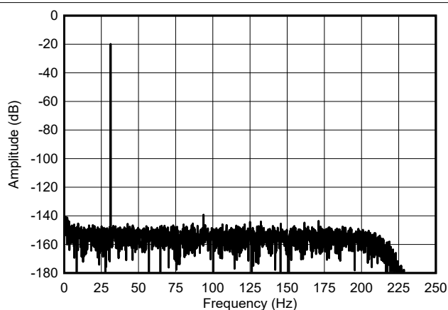
Figure 6-34. Low-Power Mode FFT Spectrum
