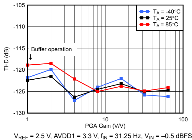
Figure 6-47. Mid-Power Mode THD vs PGA Gain
