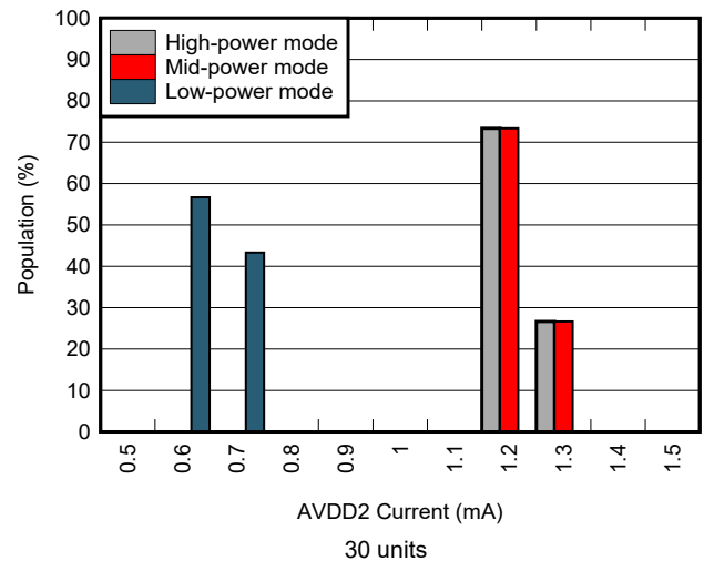
Figure 6-64. AVDD2 Current Distribution
