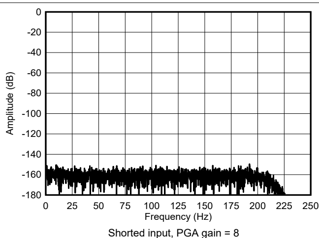
Figure 6-10. High-Power Mode FFT Spectrum
