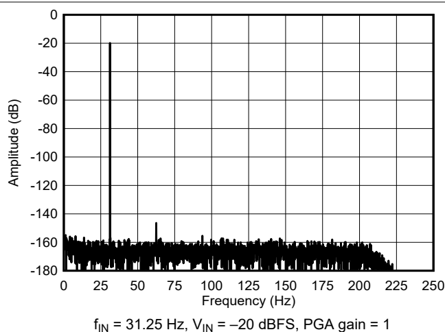
Figure 6-14. High-Power Mode FFT Spectrum
