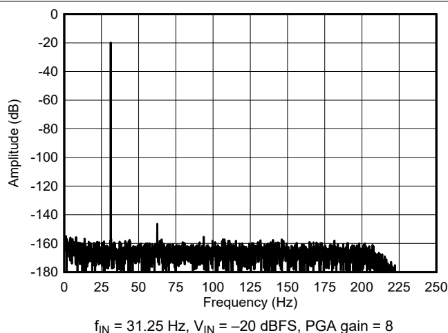
Figure 6-18. High-Power Mode FFT Spectrum
