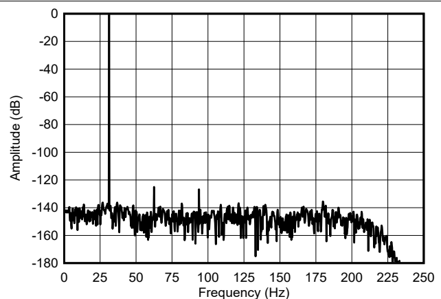
Figure 6-30. Low-Power Mode FFT Spectrum
