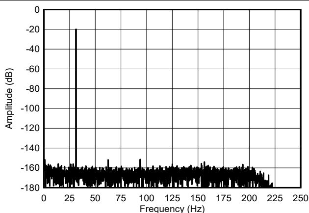
Figure 6-21. Mid-Power Mode FFT Spectrum
