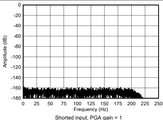
Figure 6-19. Mid-Power Mode FFT Spectrum
