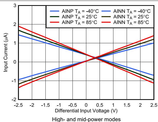
Figure 6-54. PGA Input Current vs Input Voltage
