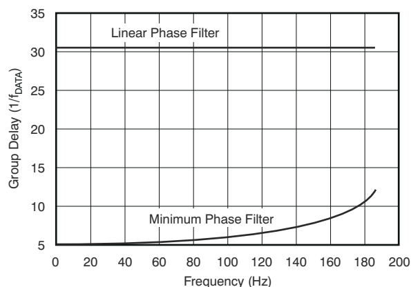
Figure 8-18. FIR Group Delay ( f_{\text{DATA}} = 500 SPS)
