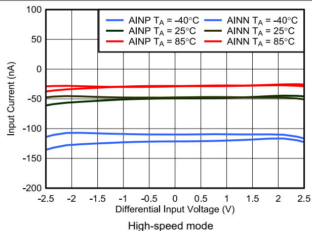
Figure 6-54. PGA Input Current vs Input Voltage
