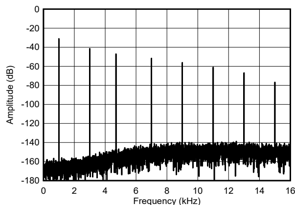
Figure 8-13. FFT Output of the Sinc Filter ( f_{\text{DATA}} = 32 kSPS)
