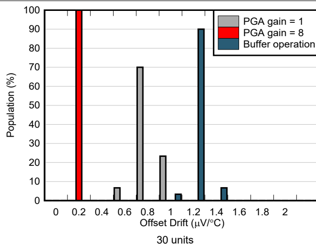
Figure 6-40. Offset Drift Distribution
