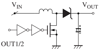
Figure 1. Output bootstrap circuit
