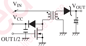
Figure 1. Output bootstrap circuit
