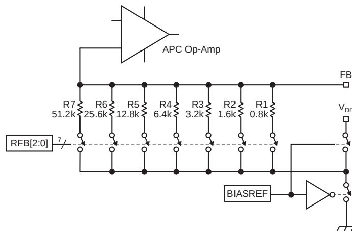
Figure 4. Programmable Feedback Resistor
