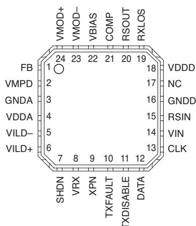
24-Pin MLF®
