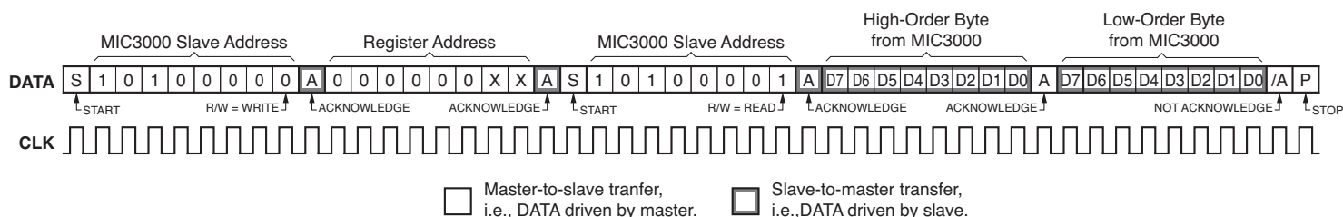
Figure 23. Read_Word Protocol
