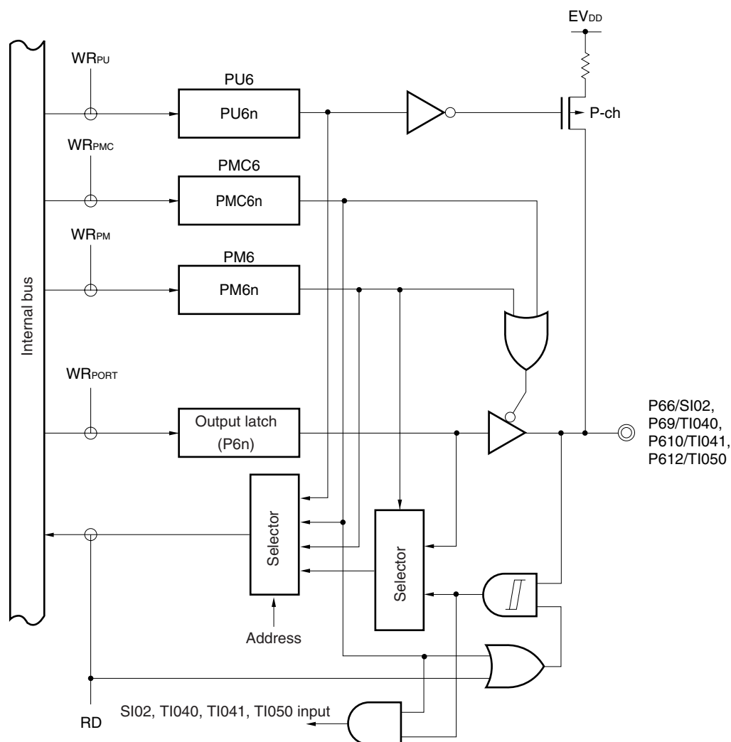
Figure 4-17. Block Diagram of P66, P69, P610, and P612
