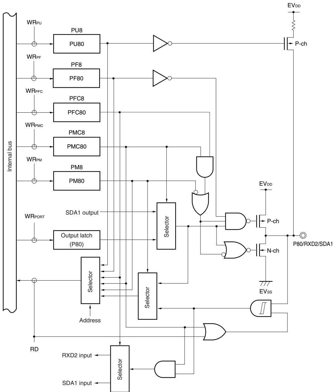
Figure 4-23. Block Diagram of P80
