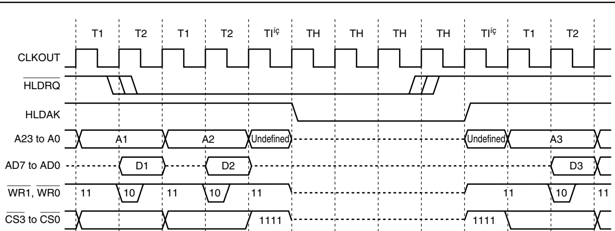
Figure 5-15. Separate Bus Hold Timing (Bus Size: 8 Bits, Write)
