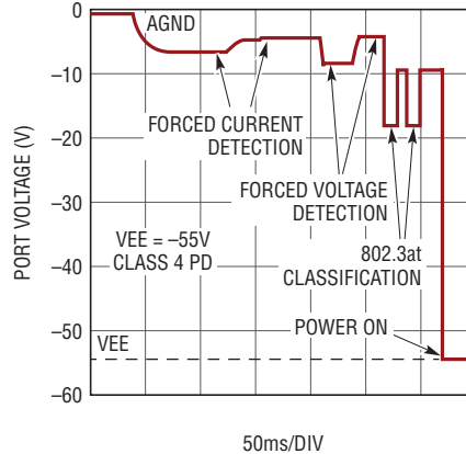
802.3at Power On Sequence in AUTO Pin Mode
