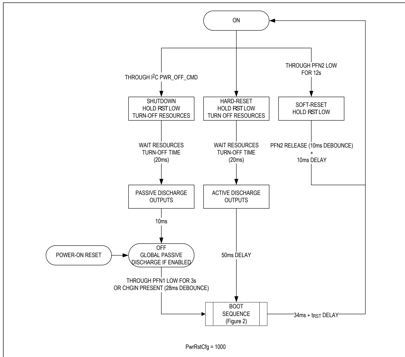
Figure 1f. PwrRstCfg = 1000
