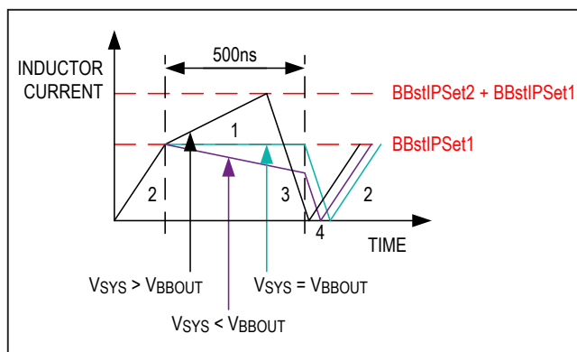
Figure 7. Buck-Boost Inductor Current in Buck-Boost Mode
