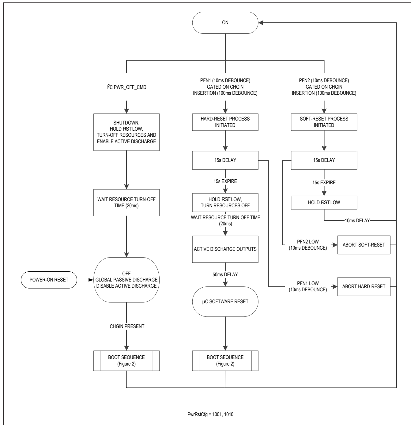
Figure 1g. PwrRstCfg = 1001, 1010
