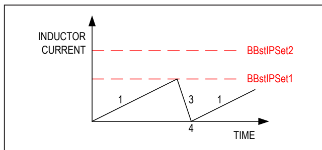
Figure 8. Buck-Boost Inductor Current in Buck-Only Mode
