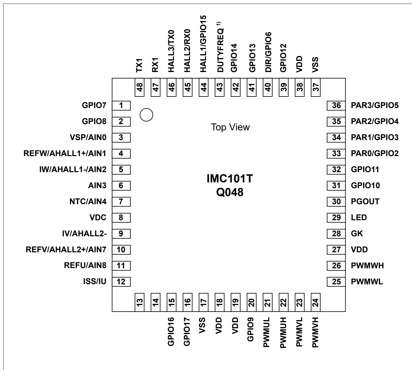
Figure 3 IMC101T-Q048
