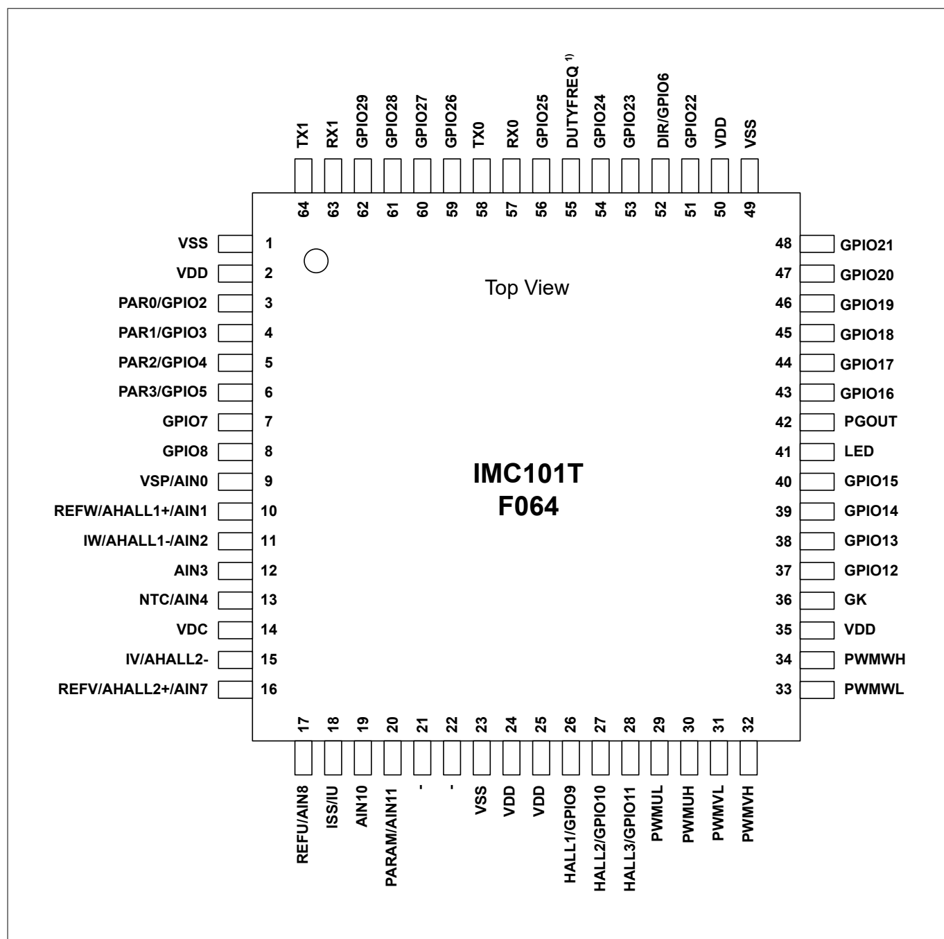
Figure 5 IMC101T-F064
