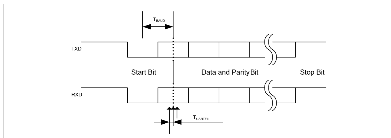
Figure 18 UART timing
