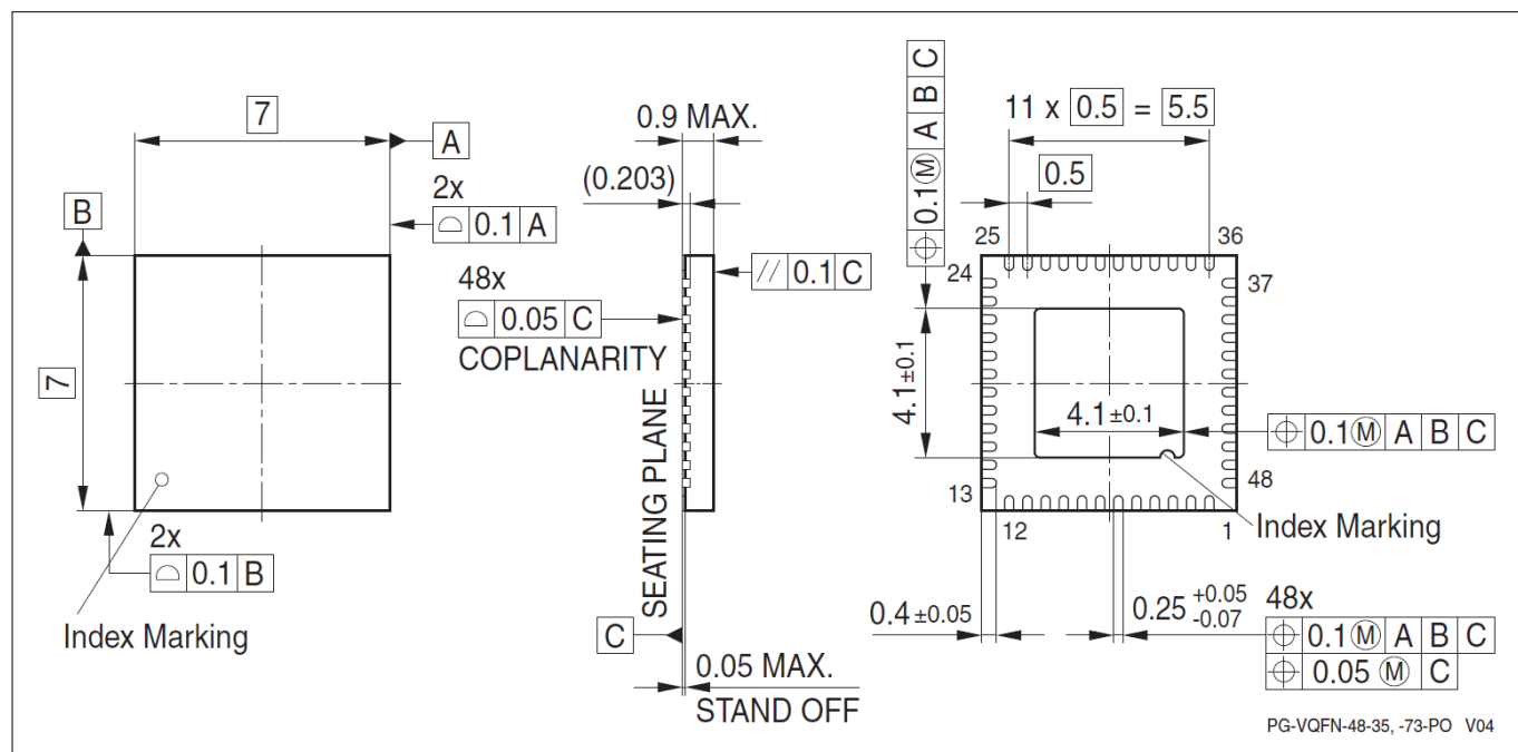
Figure 23 PG-VQFN-48-73
