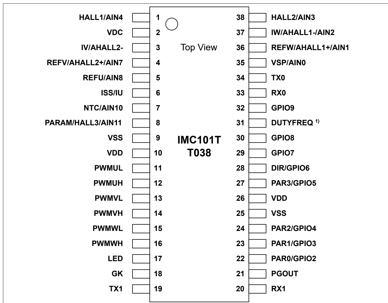
Figure 2 IMC099T-T038, IMC101T-T038
