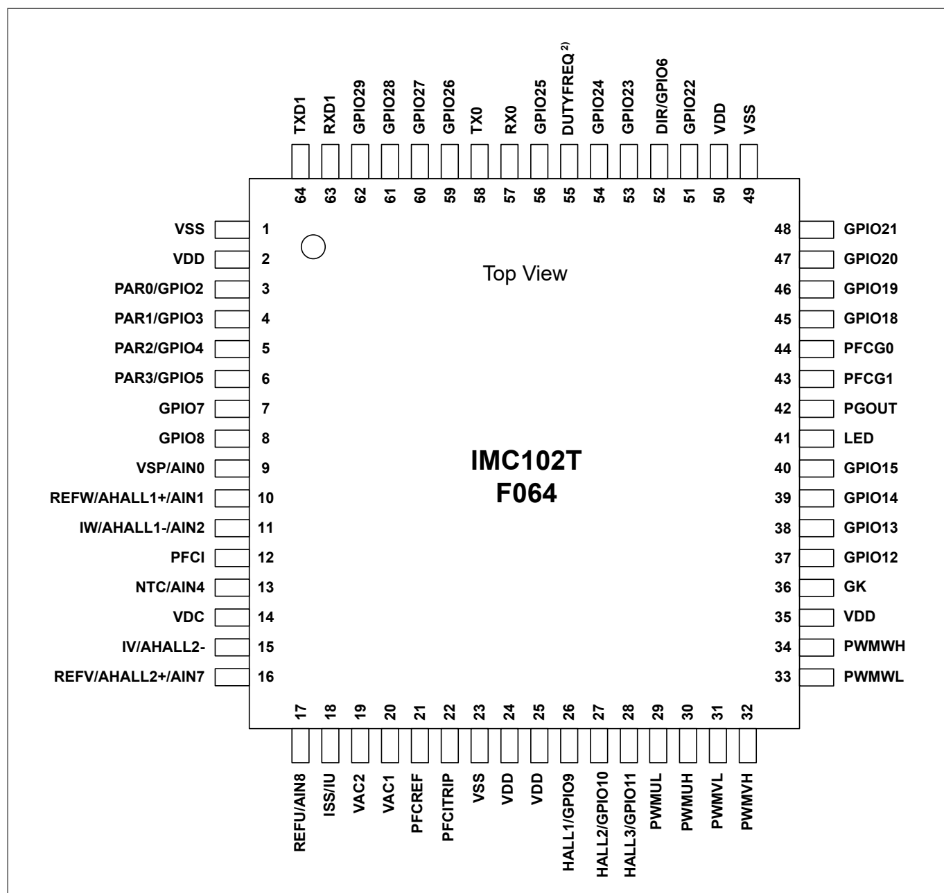
Figure 7 IMC102T-F064
