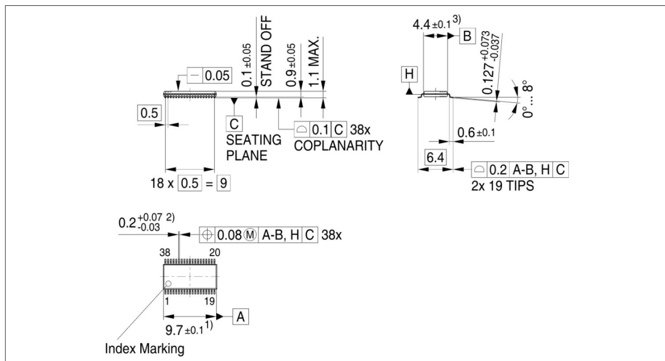
Figure 22 PG-TSSOP-38-9
