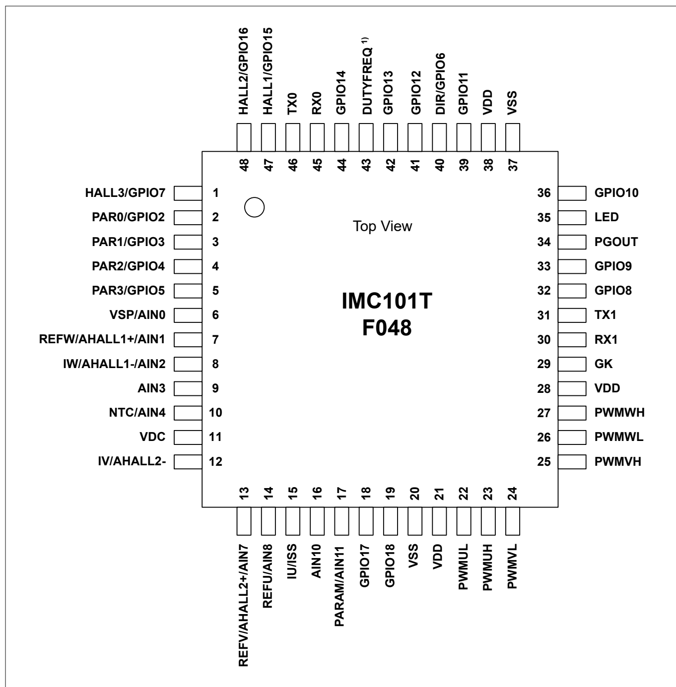
Figure 4 IMC101T-F048
