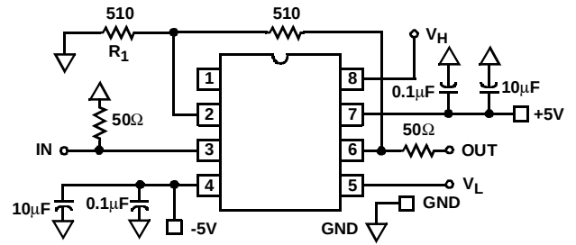
FIGURE 2C. SCHEMATIC
