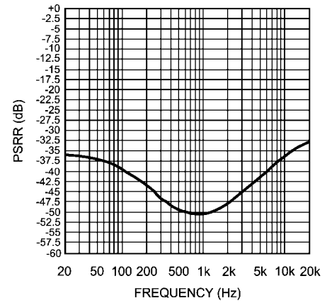
Power Supply Rejection vs Frequency V_{DD} = 3.3V , A_V = 26dB , V_{RIPPLE} = 200mV_{P-P} Input Terminated into 10\Omega
