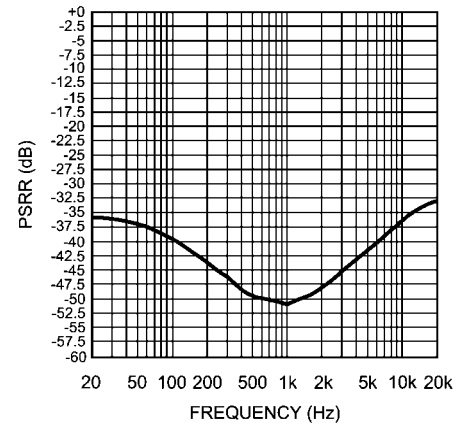
Power Supply Rejection vs Frequency V_{DD} = 5V , A_V = 26dB , V_{RIPPLE} = 200mV_{P-P} Input Terminated into 10\Omega
