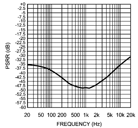
Power Supply Rejection vs Frequency V_{DD} = 7.5V , A_V = 26dB , V_{RIPPLE} = 200mV_{P-P} Input Terminated into 10\Omega
