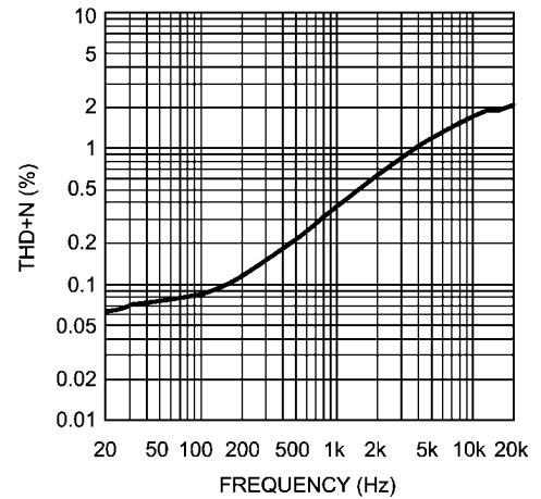
THD+N vs Frequency V_{DD} = 3.3V , P_O = 100mW , A_V = 26dB
