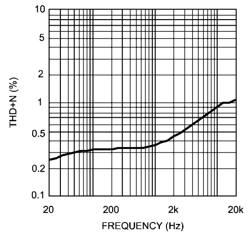
THD+N vs Frequency V_{DD} = 7.5V , P_O = 600mW , A_V = 26dB
