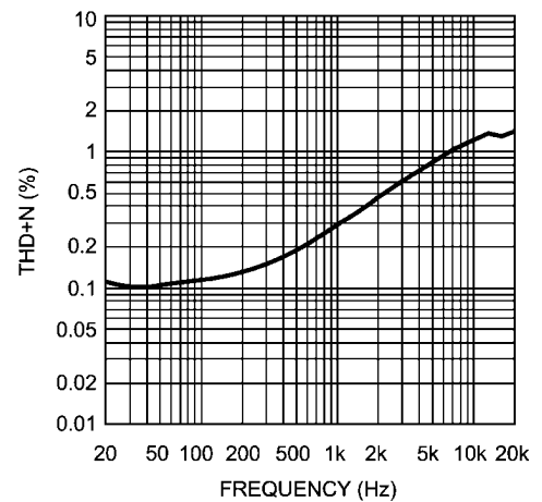
THD+N vs Frequency V_{DD} = 5V , P_O = 400mW , A_V = 26dB
