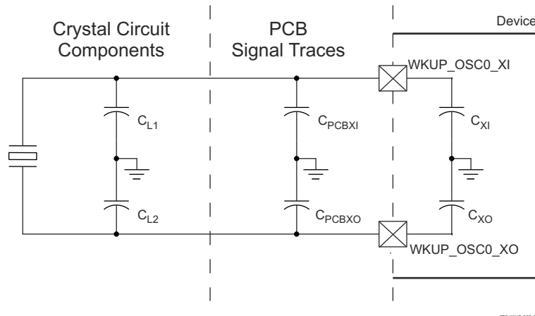
Figure 7-25. Load Capacitance
