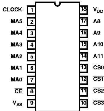
CDP1882, CDP1882C (PDIP, CERP) TOP VIEW
