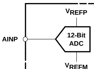
Figure 36. Single-Ended Input Stage
