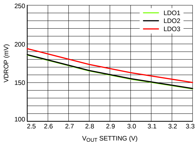
Figure 11. Dropout Voltage vs. V_{OUT} , LDO1, 2 & 3 ( I_{OUT} = 200\text{ mA} )
