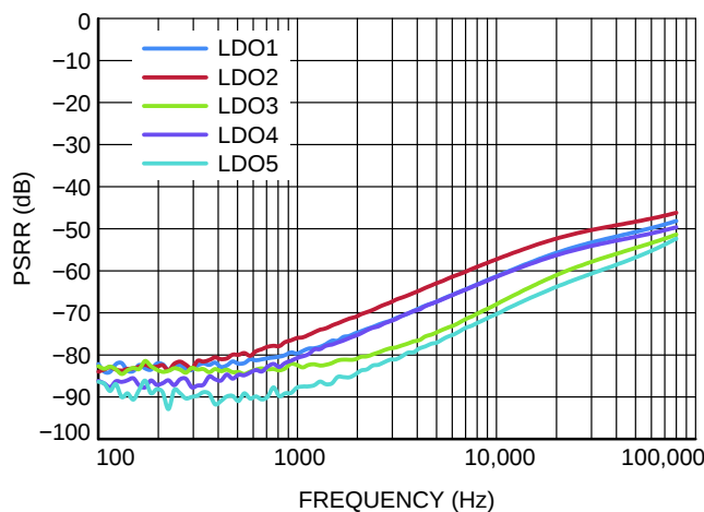
Figure 13. LDOx PSRR ( V_{IN} = 3.6\text{ V} - V_{OUT} = 1.8\text{ V} - I_{OUT} = 5\text{ mA} )
