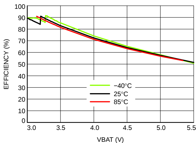
Figure 15. Torch LED Efficiency vs. Input Voltage ( I_{TORCH} = 300\text{ mA} , V_{IN} Falling)
