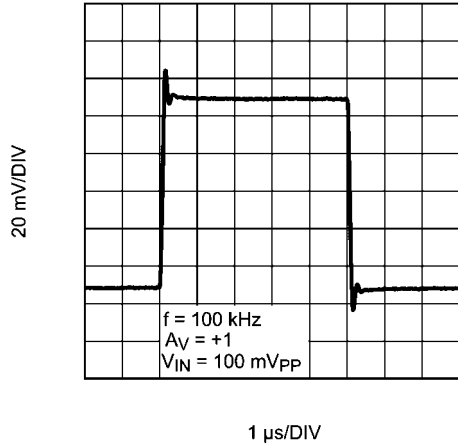
Small Signal Step Response with Gain = 1
